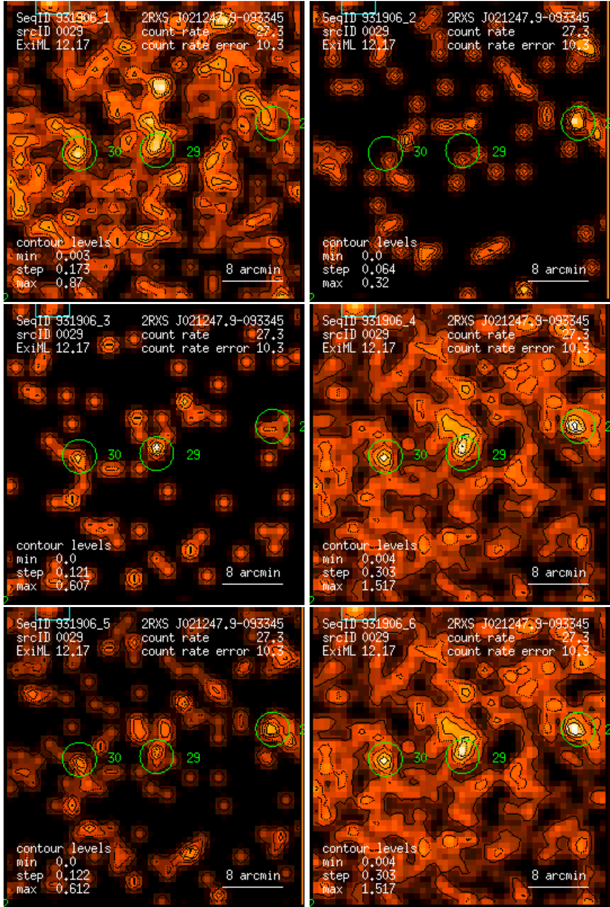
Figure 29: RASS 931906: detection 0029: band rate images, Gaussian filter: (1) PSPC channels 11 – 41, (2) 52 – 90, (3) 91 – 201, (4) 11 – 235, (5) 52 – 201, (6) 11 – 201. Broad band rates in counts/ks. Band rate contour levels in counts/ks/arcmin 2 .
