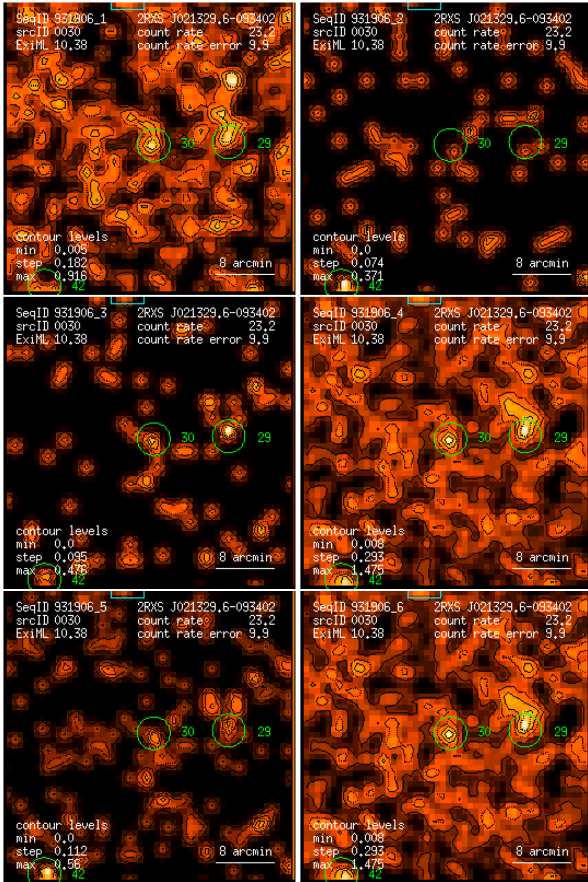
Figure 30: RASS 931906: detection 0030: band rate images, Gaussian filter: (1) PSPC channels 11 – 41, (2) 52 – 90, (3) 91 – 201, (4) 11 – 235, (5) 52 – 201, (6) 11 – 201. Broad band rates in counts/ks. Band rate contour levels in counts/ks/arcmin 2 .
