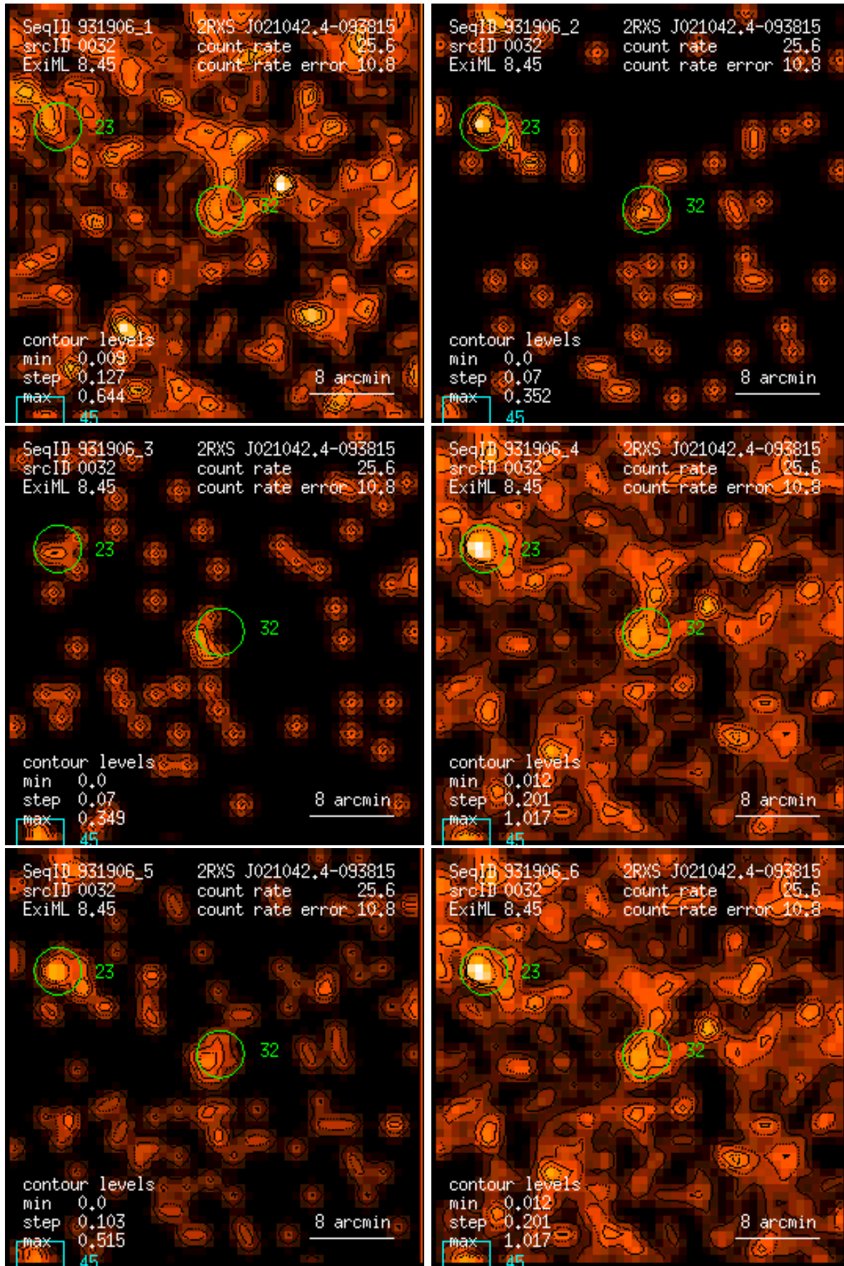
Figure 32: RASS 931906: detection 0032: band rate images, Gaussian filter: (1) PSPC channels 11 – 41, (2) 52 – 90, (3) 91 – 201, (4) 11 – 235, (5) 52 – 201, (6) 11 – 201. Broad band rates in counts/ks. Band rate contour levels in counts/ks/arcmin 2 .
