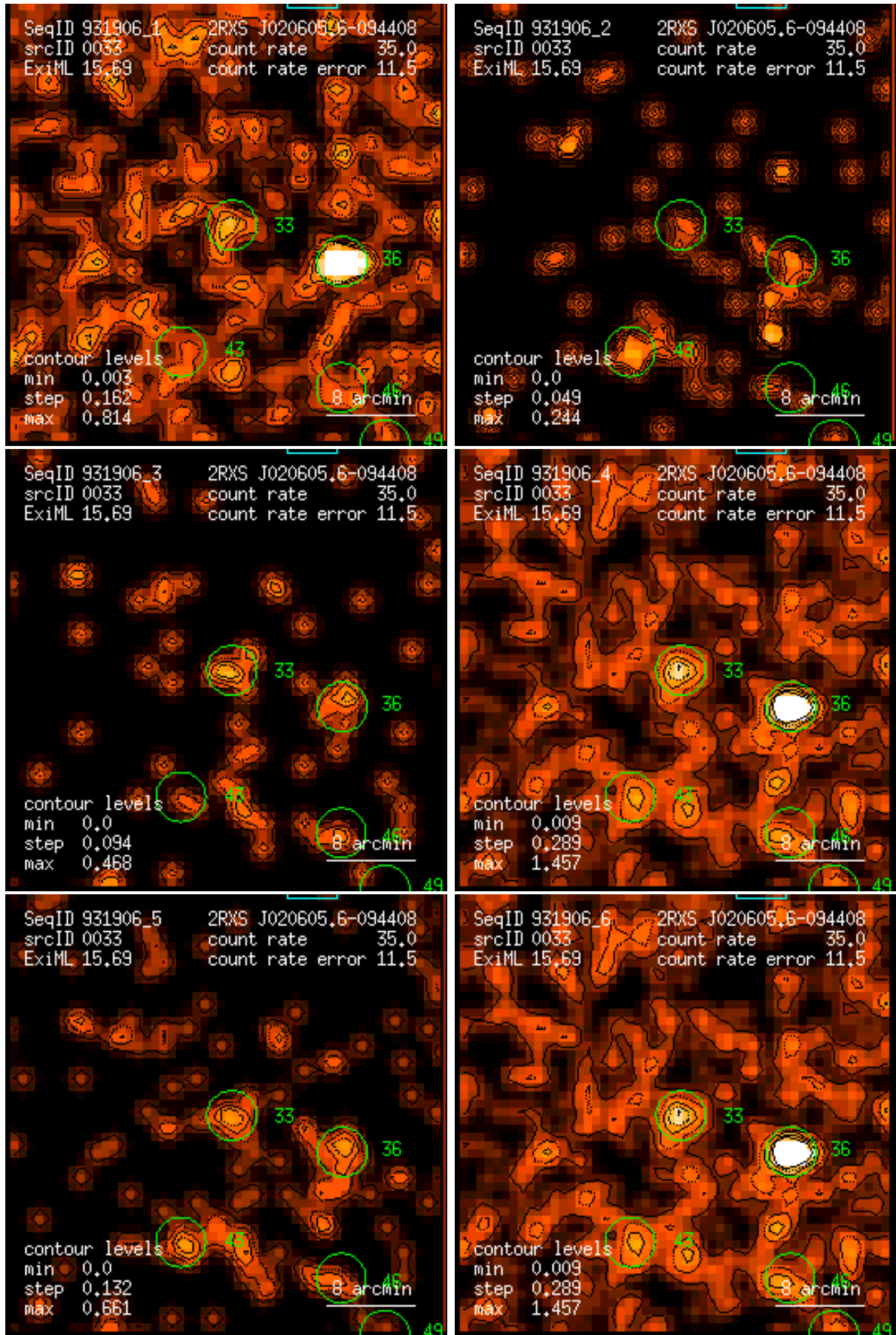
Figure 33: RASS 931906: detection 0033: band rate images, Gaussian filter: (1) PSPC channels 11 – 41, (2) 52 – 90, (3) 91 – 201, (4) 11 – 235, (5) 52 – 201, (6) 11 – 201. Broad band rates in counts/ks. Band rate contour levels in counts/ks/arcmin 2 .
