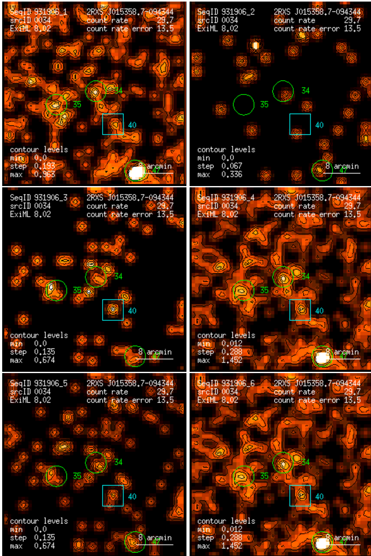
Figure 34: RASS 931906: detection 0034: band rate images, Gaussian filter: (1) PSPC channels 11 – 41, (2) 52 – 90, (3) 91 – 201, (4) 11 – 235, (5) 52 – 201, (6) 11 – 201. Broad band rates in counts/ks. Band rate contour levels in counts/ks/arcmin 2 .
