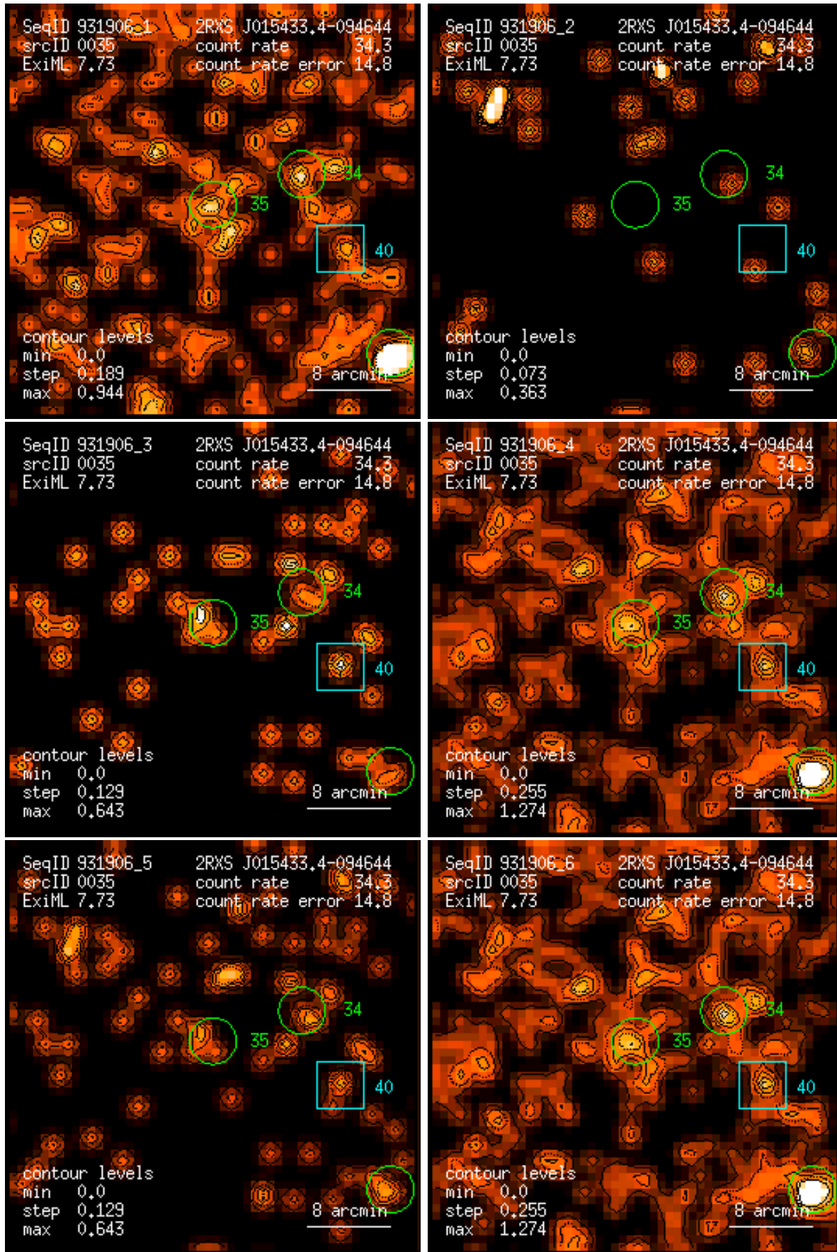
Figure 35: RASS 931906: detection 0035: band rate images, Gaussian filter: (1) PSPC channels 11 – 41, (2) 52 – 90, (3) 91 – 201, (4) 11 – 235, (5) 52 – 201, (6) 11 – 201. Broad band rates in counts/ks. Band rate contour levels in counts/ks/arcmin 2 .
