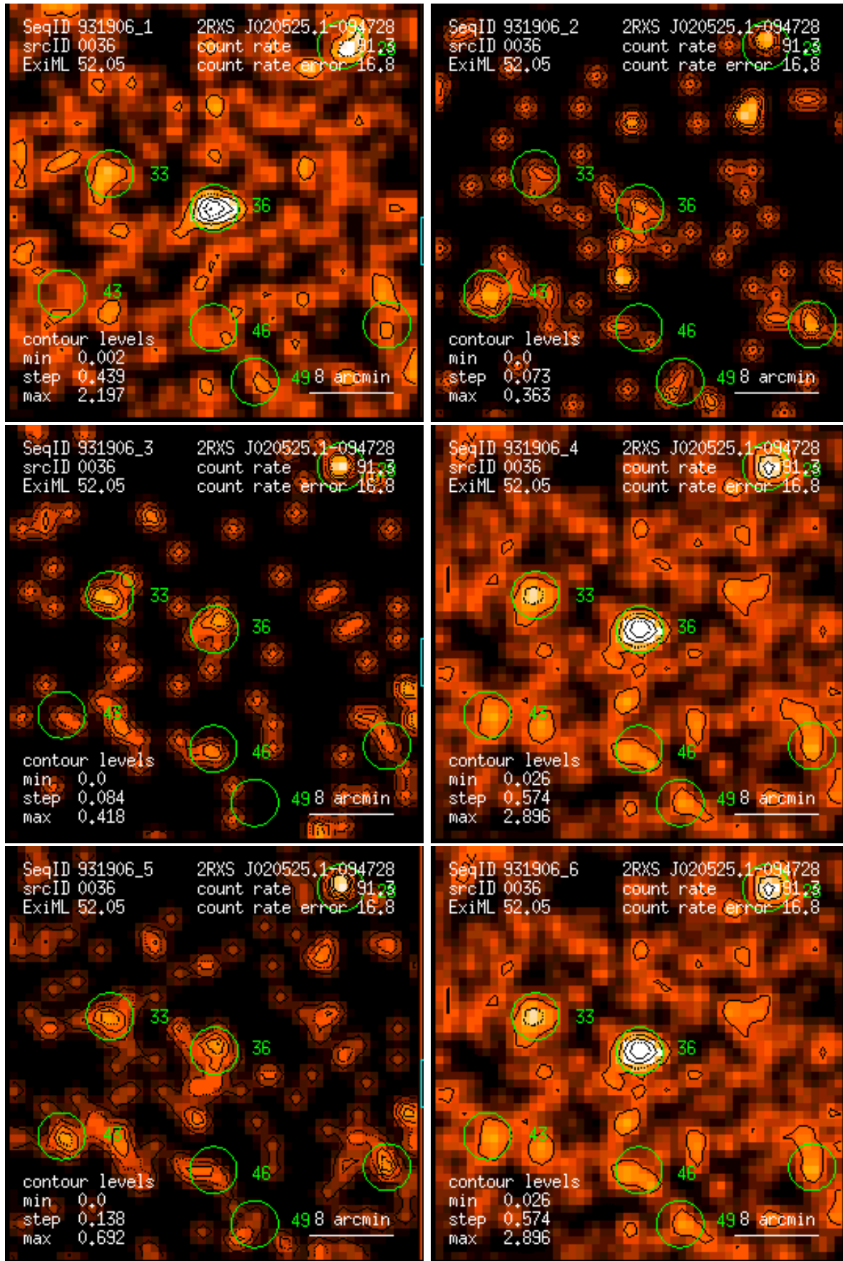
Figure 36: RASS 931906: detection 0036: band rate images, Gaussian filter: (1) PSPC channels 11 – 41, (2) 52 – 90, (3) 91 – 201, (4) 11 – 235, (5) 52 – 201, (6) 11 – 201. Broad band rates in counts/ks. Band rate contour levels in counts/ks/arcmin 2 .
