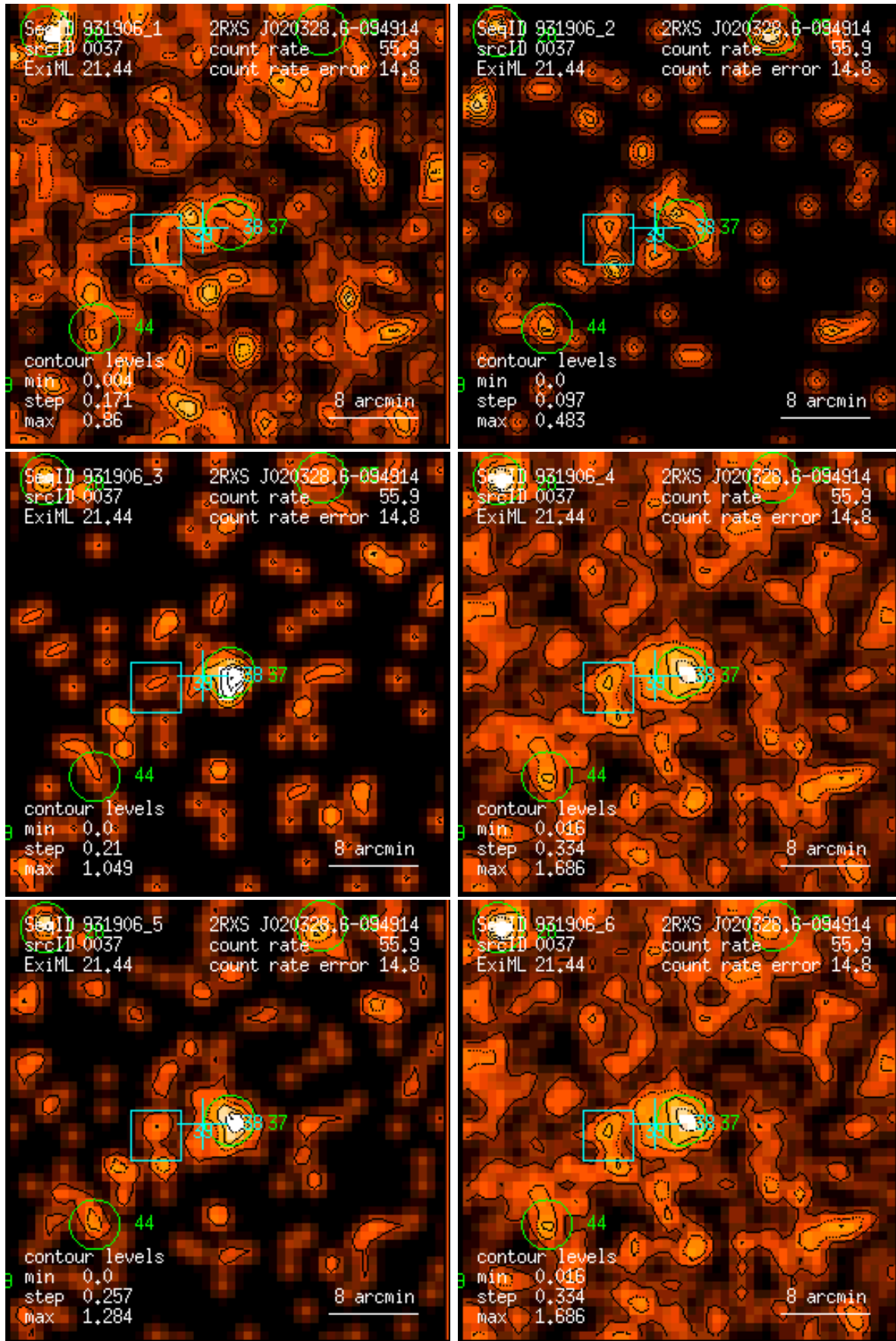
Figure 37: RASS 931906: detection 0037: band rate images, Gaussian filter: (1) PSPC channels 11 – 41, (2) 52 – 90, (3) 91 – 201, (4) 11 – 235, (5) 52 – 201, (6) 11 – 201. Broad band rates in counts/ks. Band rate contour levels in counts/ks/arcmin 2 .
