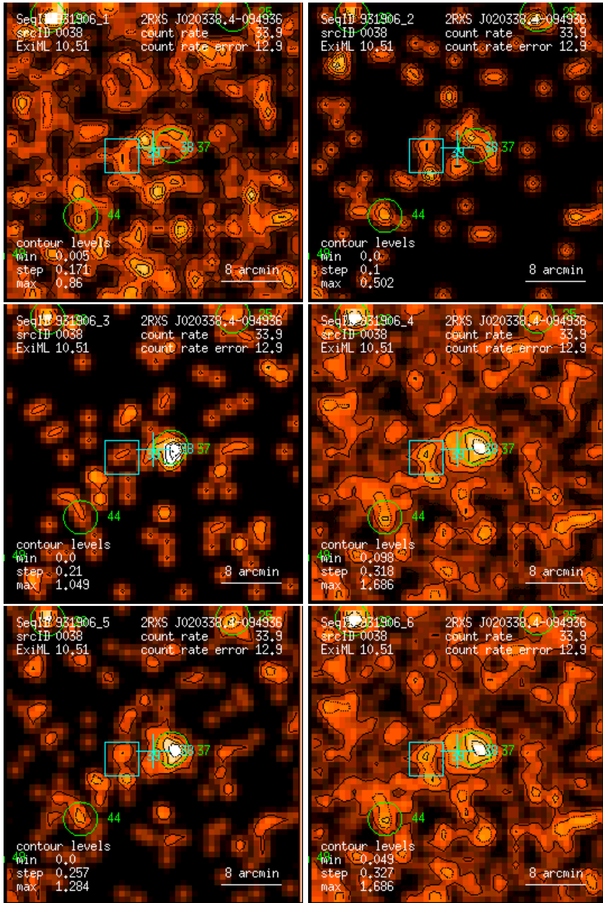
Figure 38: RASS 931906: detection 0038: band rate images, Gaussian filter: (1) PSPC channels 11 – 41, (2) 52 – 90, (3) 91 – 201, (4) 11 – 235, (5) 52 – 201, (6) 11 – 201. Broad band rates in counts/ks. Band rate contour levels in counts/ks/arcmin 2 .
