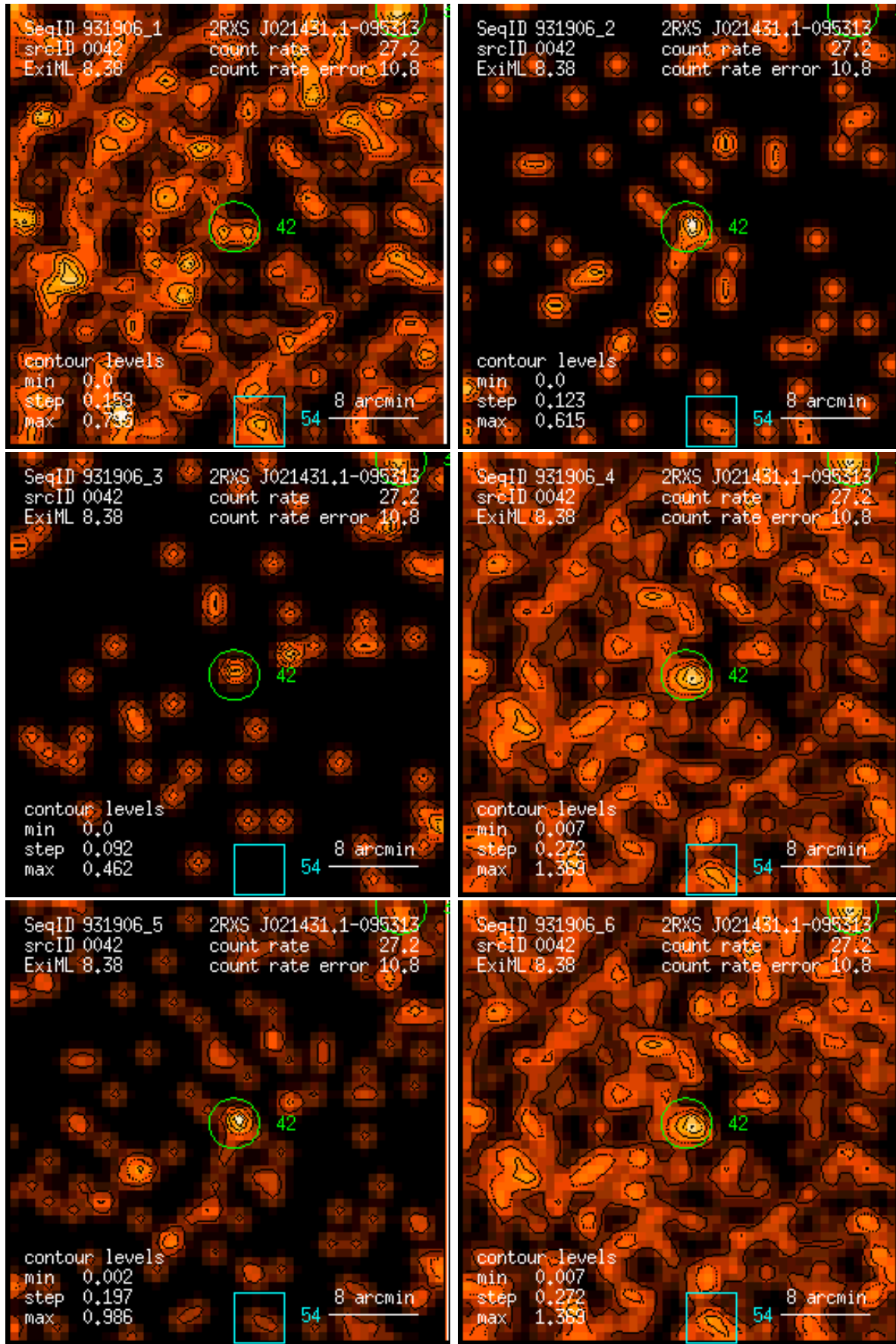
Figure 42: RASS 931906: detection 0042: band rate images, Gaussian filter: (1) PSPC channels 11 – 41, (2) 52 – 90, (3) 91 – 201, (4) 11 – 235, (5) 52 – 201, (6) 11 – 201. Broad band rates in counts/ks. Band rate contour levels in counts/ks/arcmin 2 .
