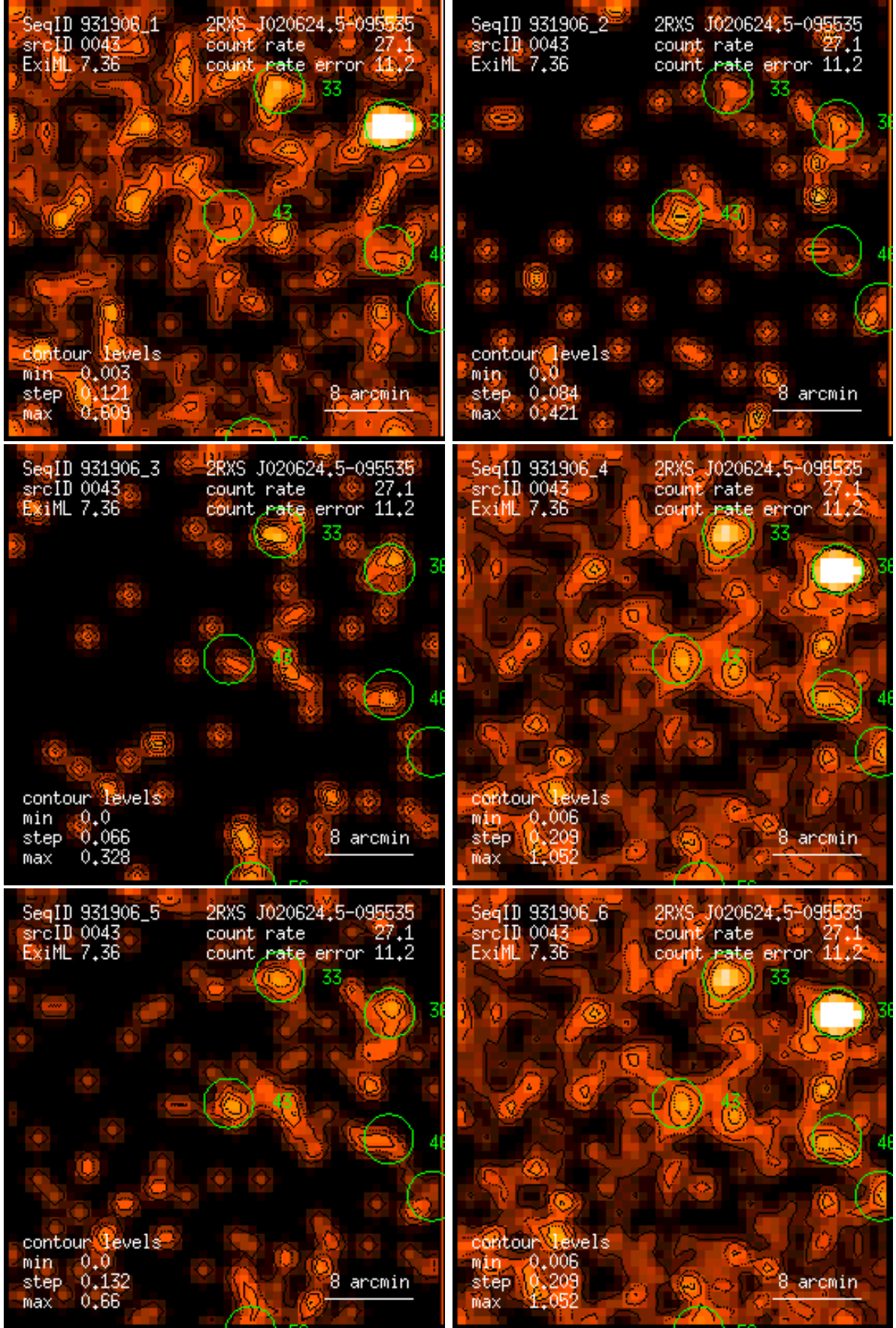
Figure 43: RASS 931906: detection 0043: band rate images, Gaussian filter: (1) PSPC channels 11 – 41, (2) 52 – 90, (3) 91 – 201, (4) 11 – 235, (5) 52 – 201, (6) 11 – 201. Broad band rates in counts/ks. Band rate contour levels in counts/ks/arcmin 2 .
