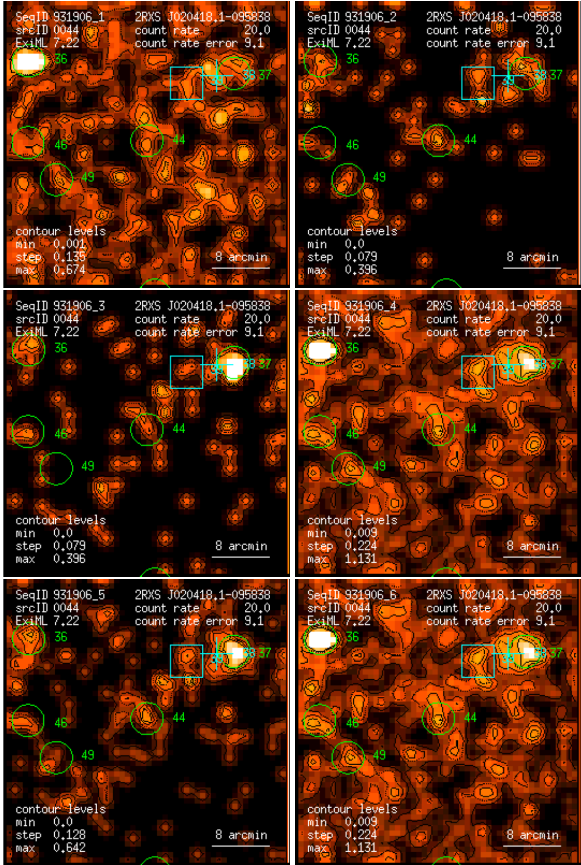
Figure 44: RASS 931906: detection 0044: band rate images, Gaussian filter: (1) PSPC channels 11 – 41, (2) 52 – 90, (3) 91 – 201, (4) 11 – 235, (5) 52 – 201, (6) 11 – 201. Broad band rates in counts/ks. Band rate contour levels in counts/ks/arcmin 2 .
