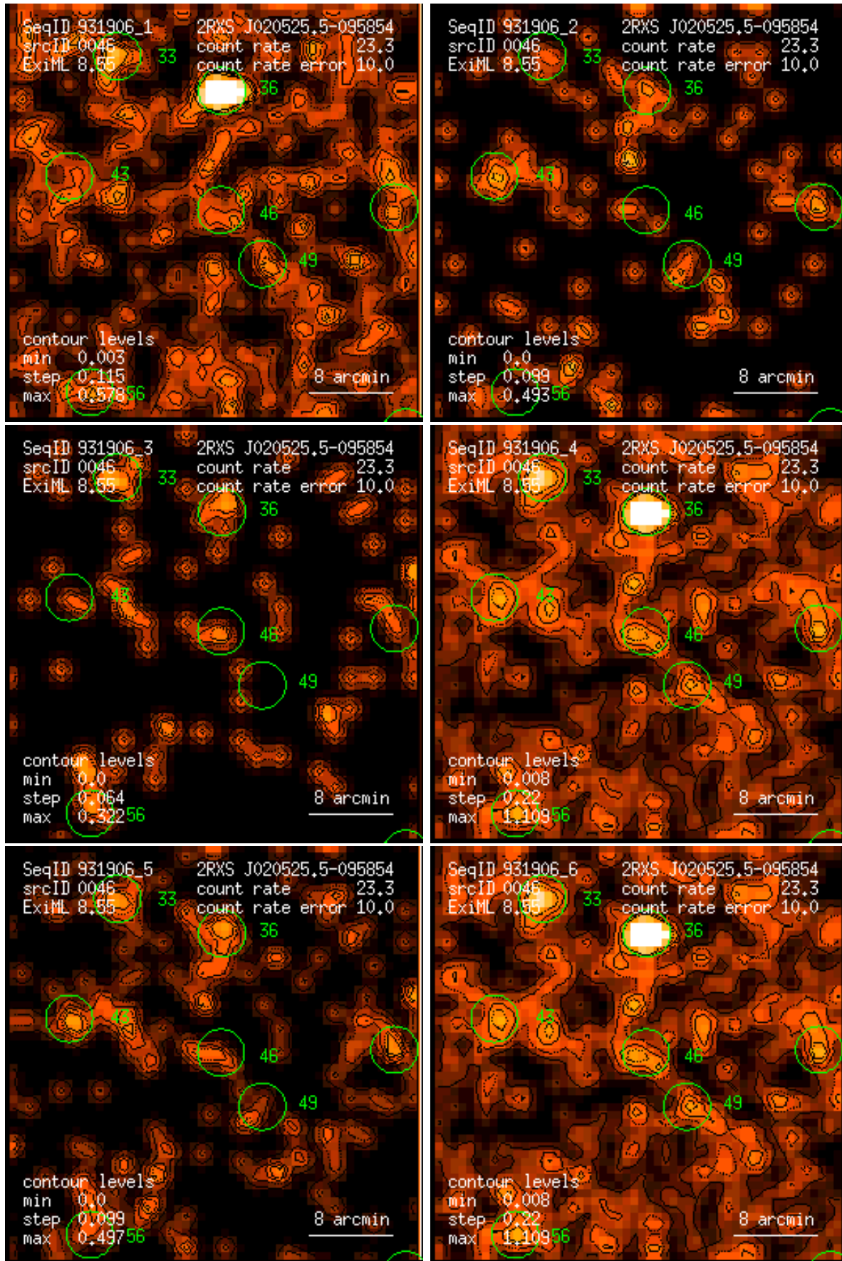
Figure 46: RASS 931906: detection 0046: band rate images, Gaussian filter: (1) PSPC channels 11 – 41, (2) 52 – 90, (3) 91 – 201, (4) 11 – 235, (5) 52 – 201, (6) 11 – 201. Broad band rates in counts/ks. Band rate contour levels in counts/ks/arcmin 2 .
