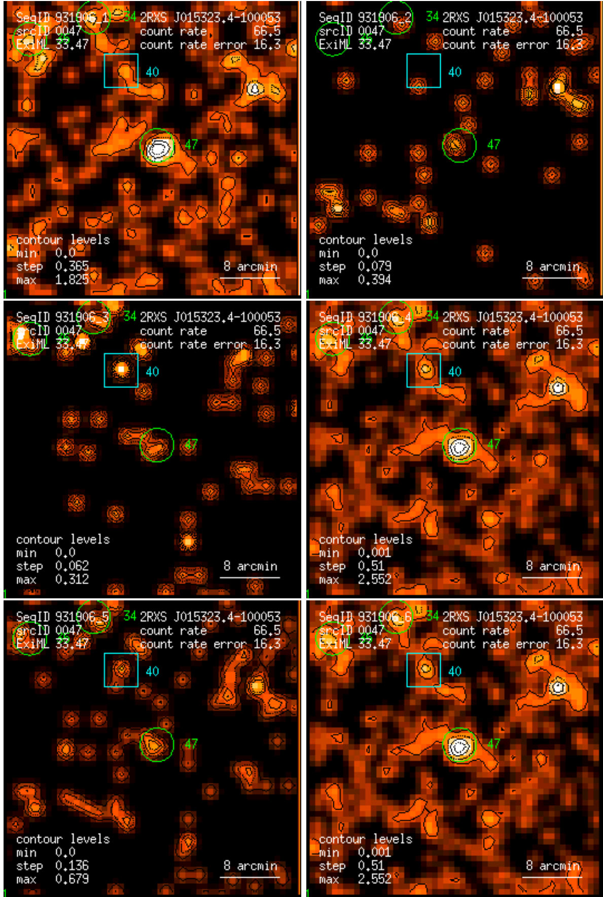
Figure 47: RASS 931906: detection 0047: band rate images, Gaussian filter: (1) PSPC channels 11 – 41, (2) 52 – 90, (3) 91 – 201, (4) 11 – 235, (5) 52 – 201, (6) 11 – 201. Broad band rates in counts/ks. Band rate contour levels in counts/ks/arcmin 2 .
