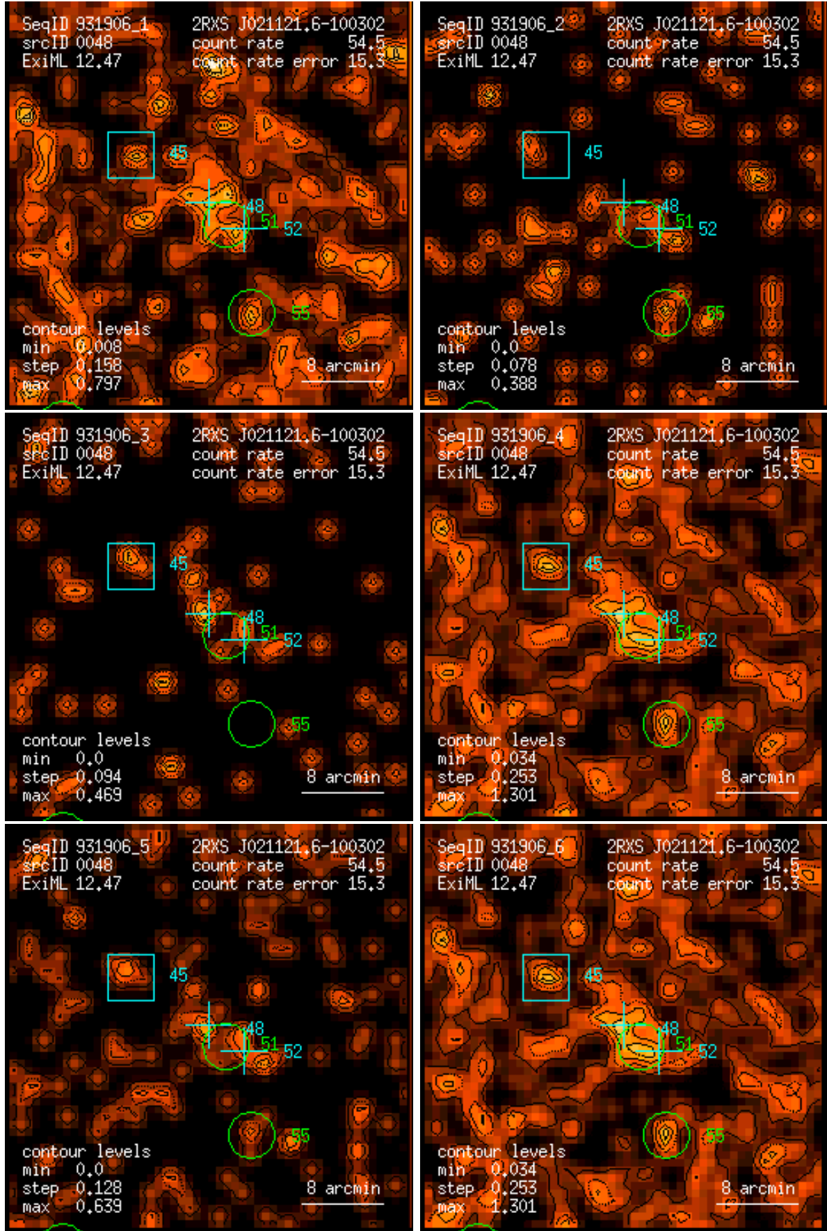
Figure 48: RASS 931906: detection 0048: band rate images, Gaussian filter: (1) PSPC channels 11 – 41, (2) 52 – 90, (3) 91 – 201, (4) 11 – 235, (5) 52 – 201, (6) 11 – 201. Broad band rates in counts/ks. Band rate contour levels in counts/ks/arcmin 2 .
