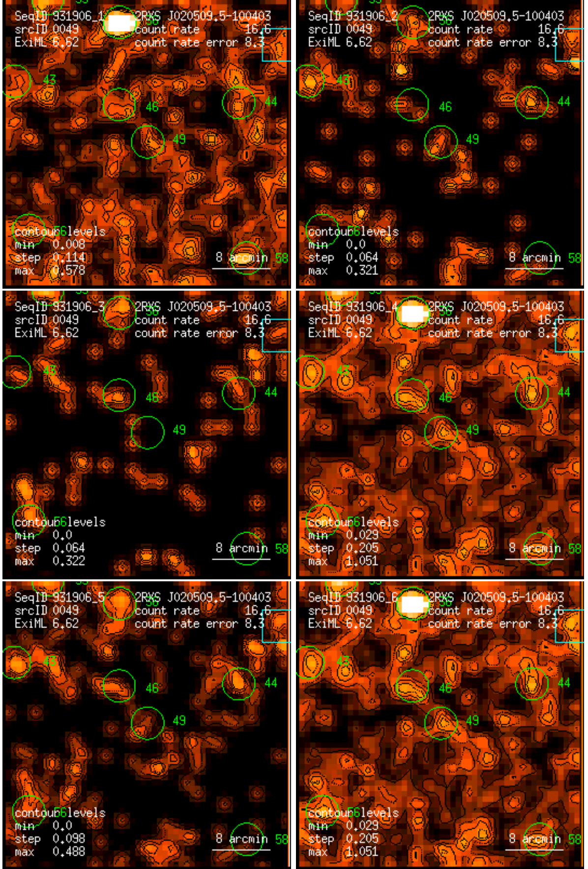
Figure 49: RASS 931906: detection 0049: band rate images, Gaussian filter: (1) PSPC channels 11 – 41, (2) 52 – 90, (3) 91 – 201, (4) 11 – 235, (5) 52 – 201, (6) 11 – 201. Broad band rates in counts/ks. Band rate contour levels in counts/ks/arcmin 2 .
