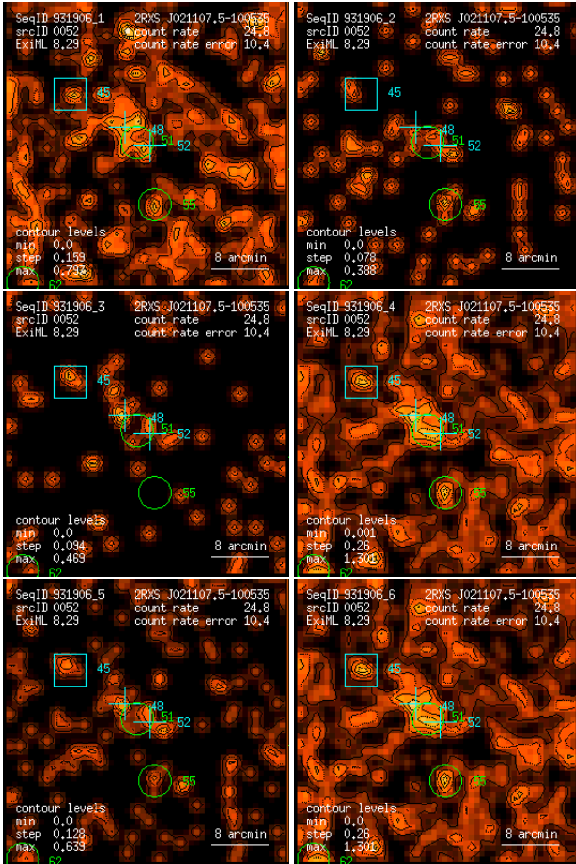
Figure 52: RASS 931906: detection 0052: band rate images, Gaussian filter: (1) PSPC channels 11 – 41, (2) 52 – 90, (3) 91 – 201, (4) 11 – 235, (5) 52 – 201, (6) 11 – 201. Broad band rates in counts/ks. Band rate contour levels in counts/ks/arcmin 2 .
