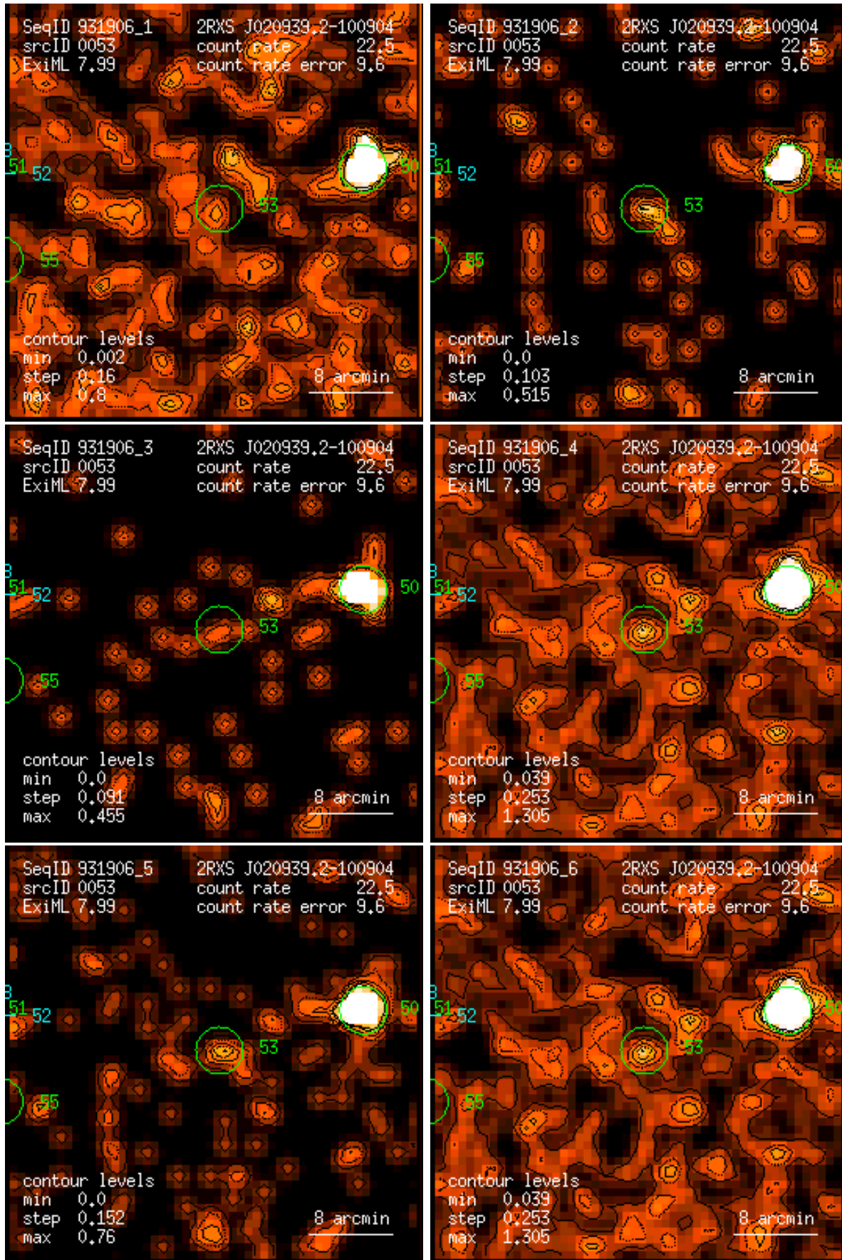
Figure 53: RASS 931906: detection 0053: band rate images, Gaussian filter: (1) PSPC channels 11 – 41, (2) 52 – 90, (3) 91 – 201, (4) 11 – 235, (5) 52 – 201, (6) 11 – 201. Broad band rates in counts/ks. Band rate contour levels in counts/ks/arcmin 2 .
