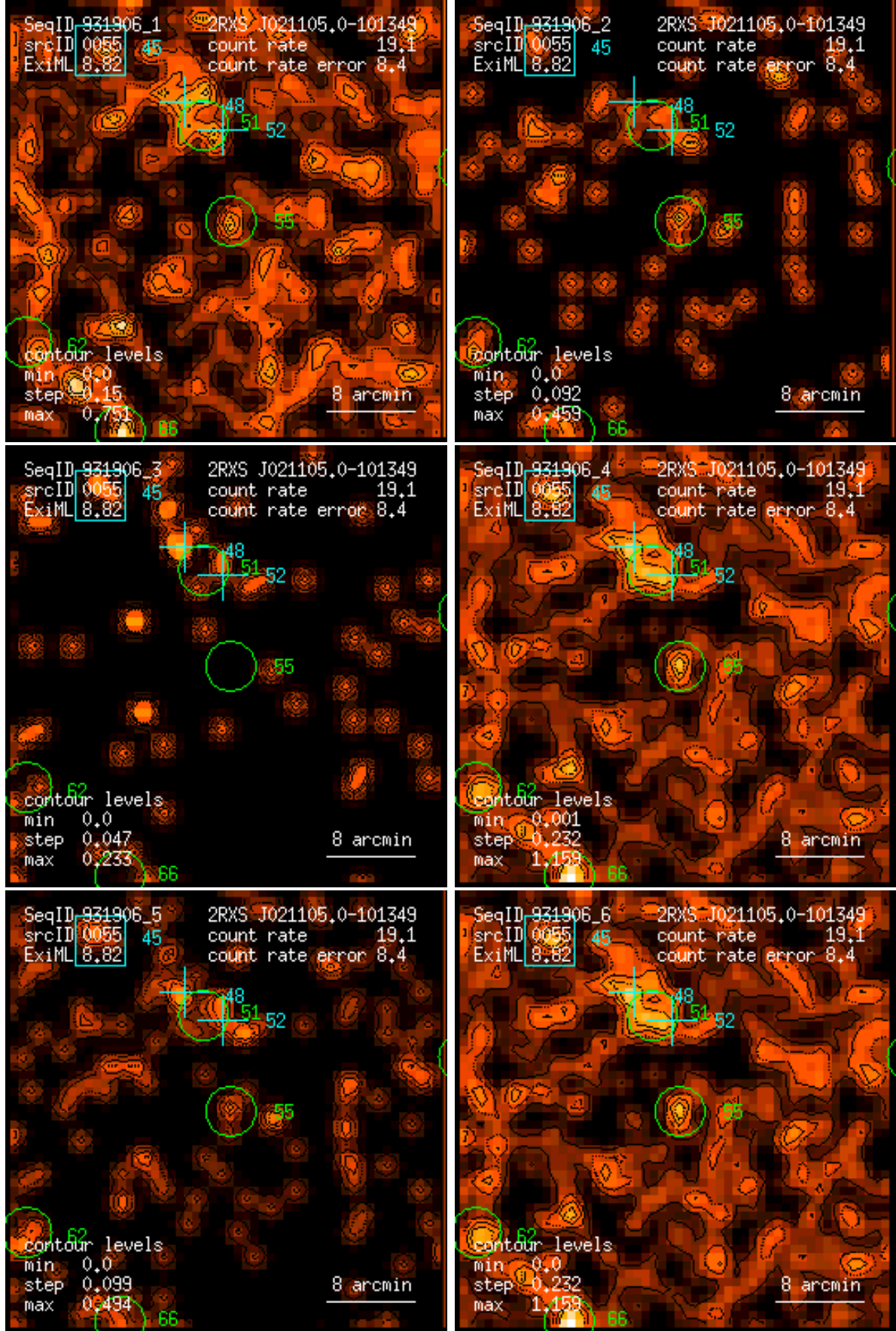
Figure 55: RASS 931906: detection 0055: band rate images, Gaussian filter: (1) PSPC channels 11 – 41, (2) 52 – 90, (3) 91 – 201, (4) 11 – 235, (5) 52 – 201, (6) 11 – 201. Broad band rates in counts/ks. Band rate contour levels in counts/ks/arcmin 2 .
