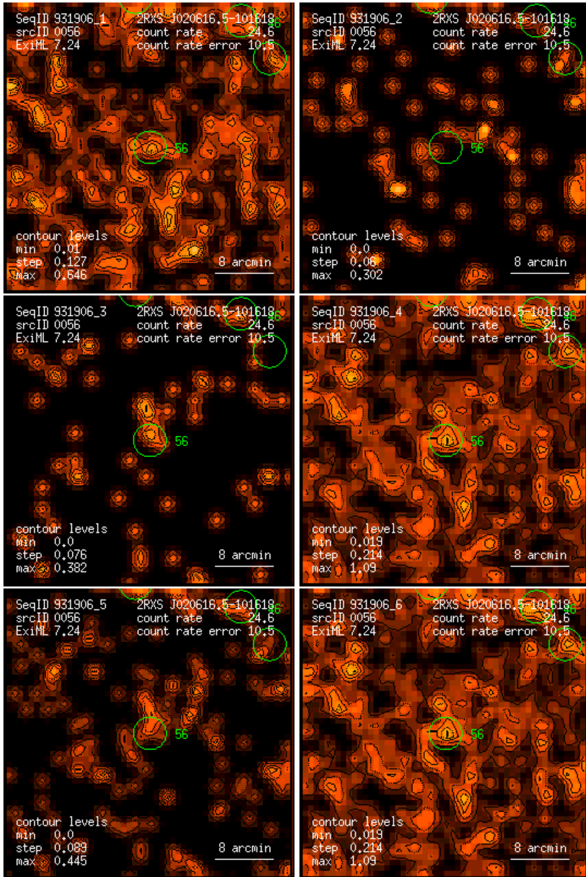
Figure 56: RASS 931906: detection 0056: band rate images, Gaussian filter: (1) PSPC channels 11 – 41, (2) 52 – 90, (3) 91 – 201, (4) 11 – 235, (5) 52 – 201, (6) 11 – 201. Broad band rates in counts/ks. Band rate contour levels in counts/ks/arcmin 2 .
