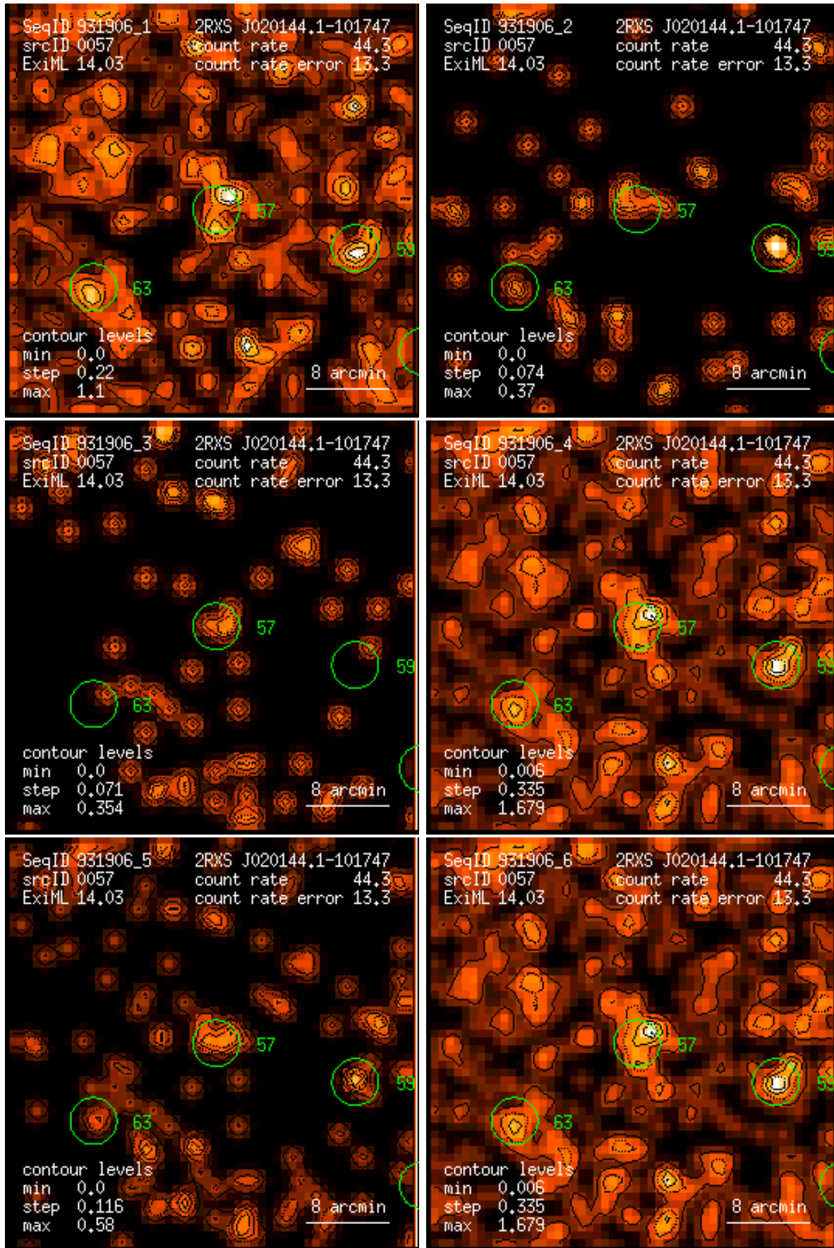
Figure 57: RASS 931906: detection 0057: band rate images, Gaussian filter: (1) PSPC channels 11 – 41, (2) 52 – 90, (3) 91 – 201, (4) 11 – 235, (5) 52 – 201, (6) 11 – 201. Broad band rates in counts/ks. Band rate contour levels in counts/ks/arcmin 2 .
