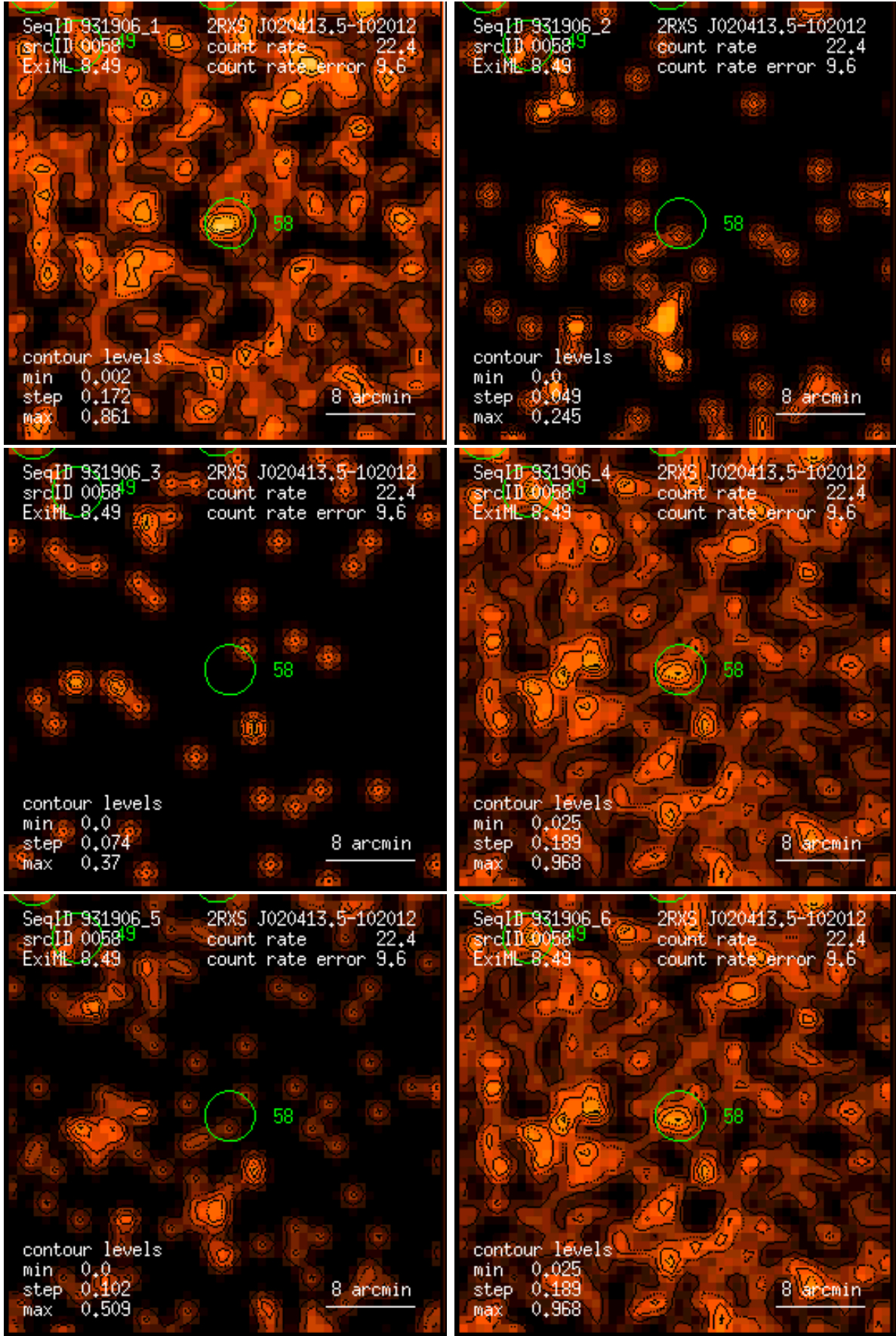
Figure 58: RASS 931906: detection 0058: band rate images, Gaussian filter: (1) PSPC channels 11 – 41, (2) 52 – 90, (3) 91 – 201, (4) 11 – 235, (5) 52 – 201, (6) 11 – 201. Broad band rates in counts/ks. Band rate contour levels in counts/ks/arcmin 2 .
