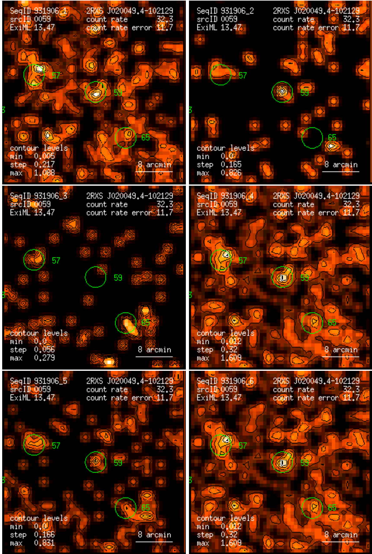
Figure 59: RASS 931906: detection 0059: band rate images, Gaussian filter: (1) PSPC channels 11 – 41, (2) 52 – 90, (3) 91 – 201, (4) 11 – 235, (5) 52 – 201, (6) 11 – 201. Broad band rates in counts/ks. Band rate contour levels in counts/ks/arcmin 2 .
