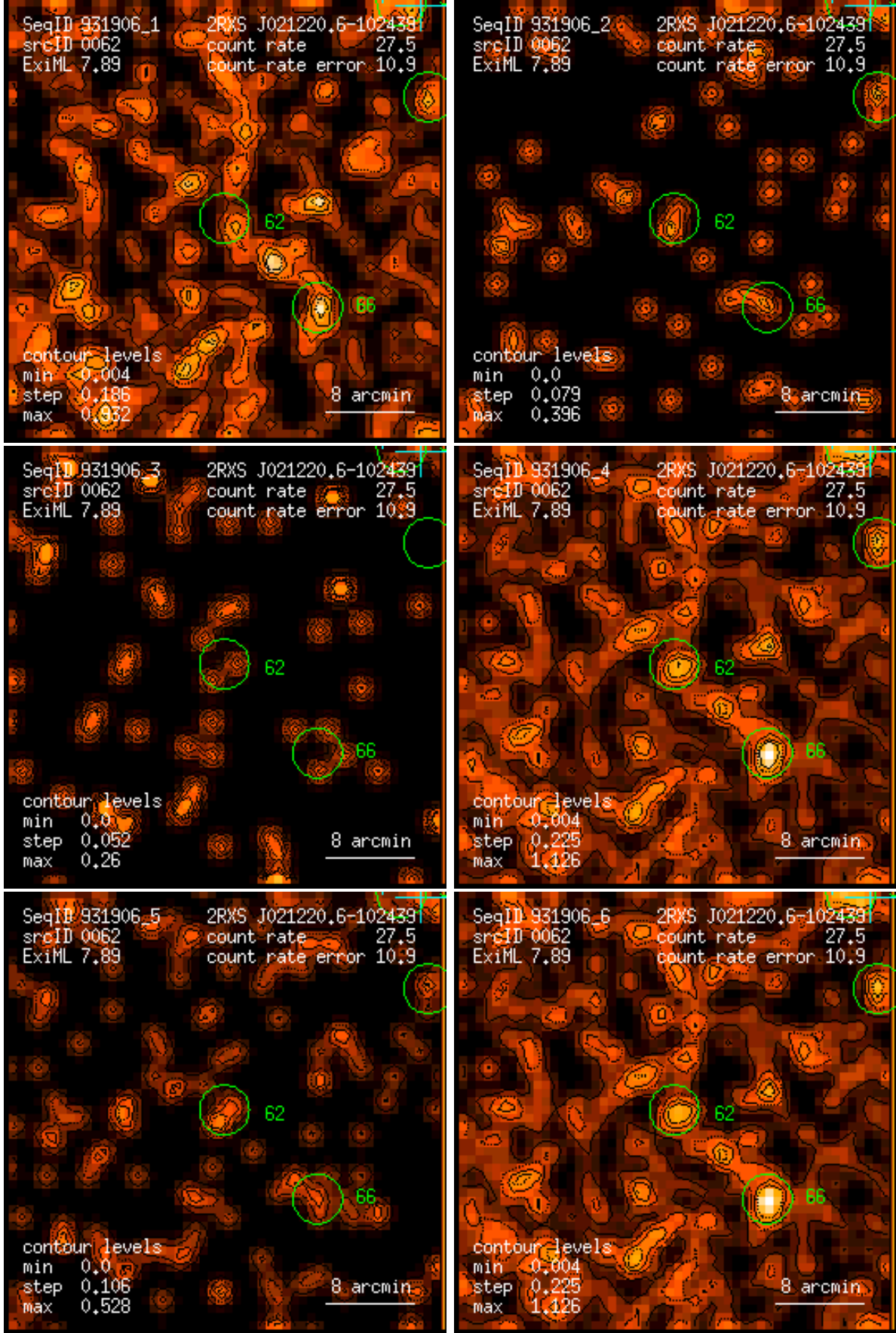
Figure 62: RASS 931906: detection 0062: band rate images, Gaussian filter: (1) PSPC channels 11 – 41, (2) 52 – 90, (3) 91 – 201, (4) 11 – 235, (5) 52 – 201, (6) 11 – 201. Broad band rates in counts/ks. Band rate contour levels in counts/ks/arcmin 2 .
