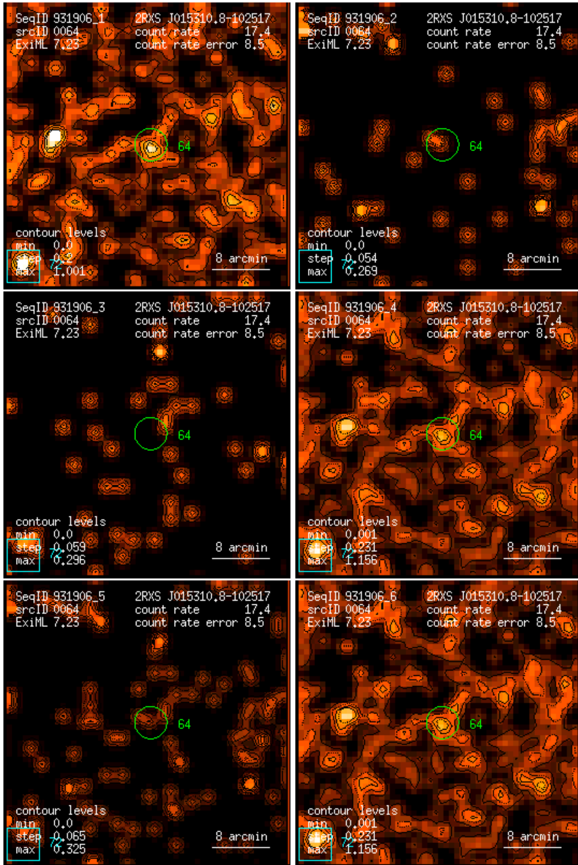
Figure 64: RASS 931906: detection 0064: band rate images, Gaussian filter: (1) PSPC channels 11 – 41, (2) 52 – 90, (3) 91 – 201, (4) 11 – 235, (5) 52 – 201, (6) 11 – 201. Broad band rates in counts/ks. Band rate contour levels in counts/ks/arcmin 2 .
