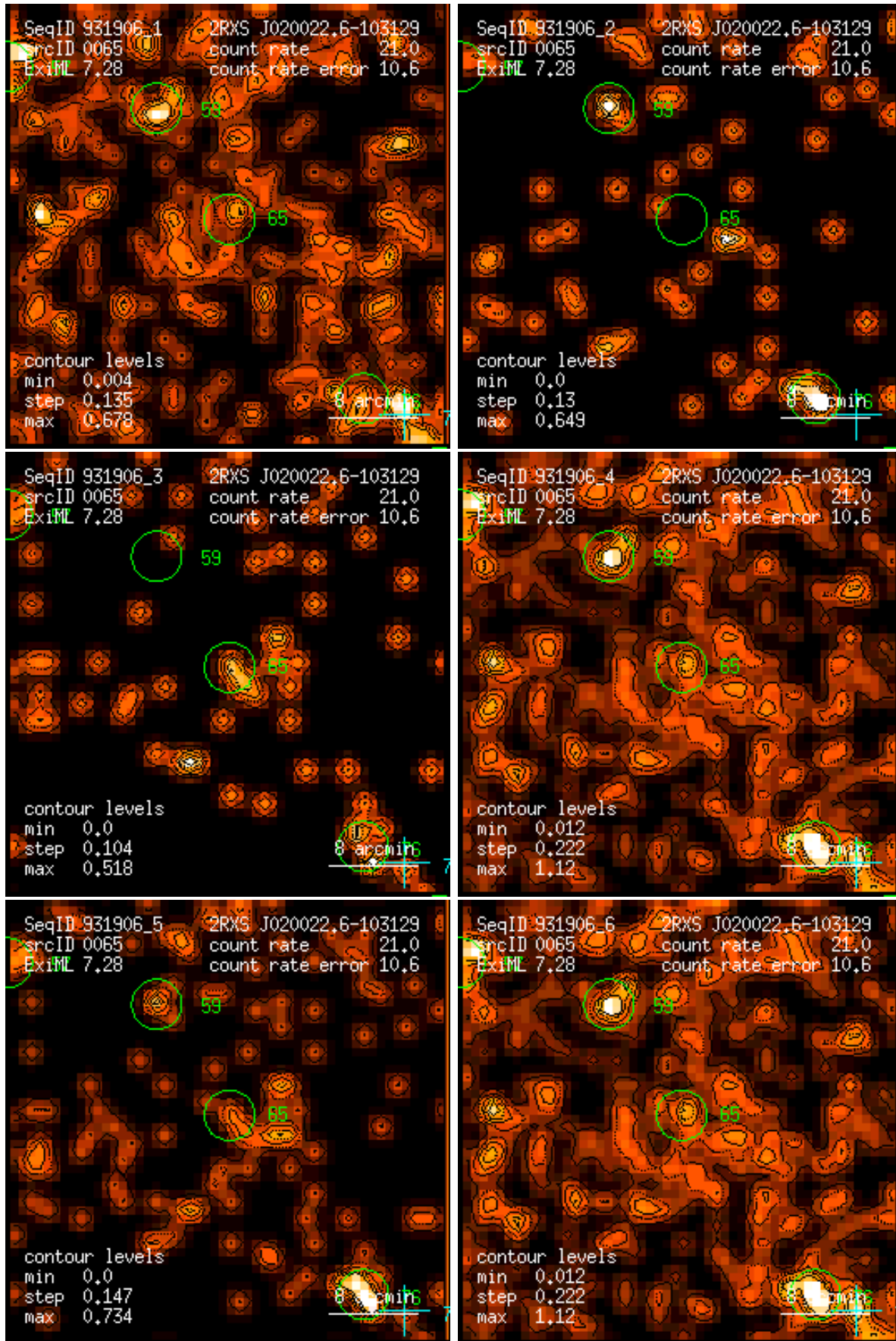
Figure 65: RASS 931906: detection 0065: band rate images, Gaussian filter: (1) PSPC channels 11 – 41, (2) 52 – 90, (3) 91 – 201, (4) 11 – 235, (5) 52 – 201, (6) 11 – 201. Broad band rates in counts/ks. Band rate contour levels in counts/ks/arcmin 2 .
