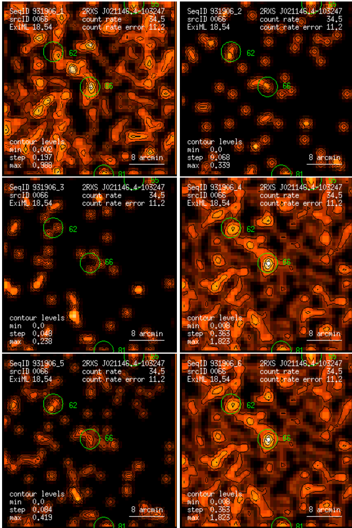
Figure 66: RASS 931906: detection 0066: band rate images, Gaussian filter: (1) PSPC channels 11 – 41, (2) 52 – 90, (3) 91 – 201, (4) 11 – 235, (5) 52 – 201, (6) 11 – 201. Broad band rates in counts/ks. Band rate contour levels in counts/ks/arcmin 2 .
