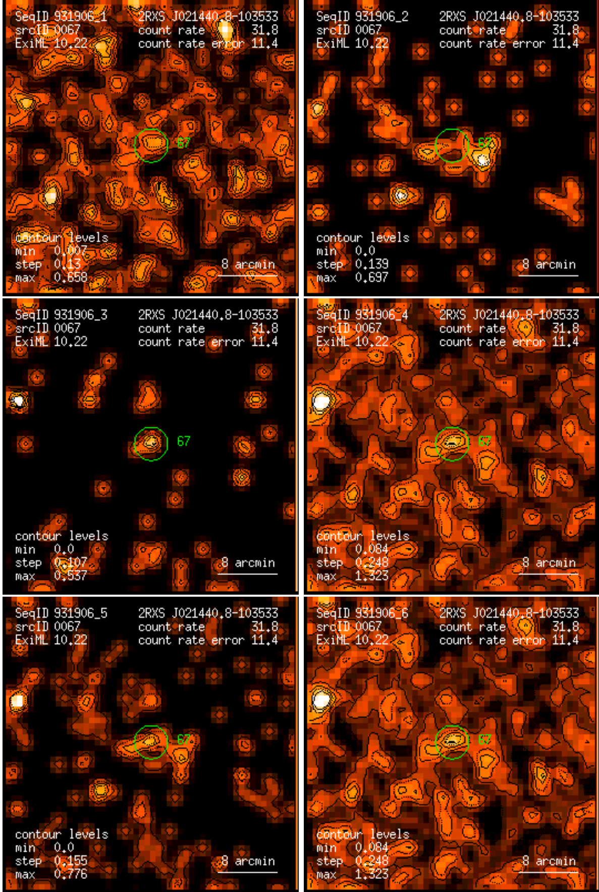
Figure 67: RASS 931906: detection 0067: band rate images, Gaussian filter: (1) PSPC channels 11 – 41, (2) 52 – 90, (3) 91 – 201, (4) 11 – 235, (5) 52 – 201, (6) 11 – 201. Broad band rates in counts/ks. Band rate contour levels in counts/ks/arcmin 2 .
