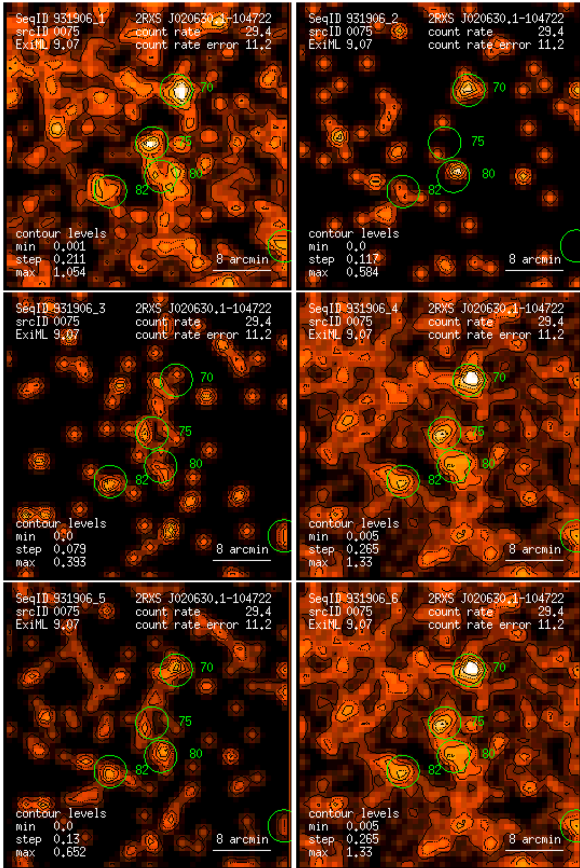
Figure 75: RASS 931906: detection 0075: band rate images, Gaussian filter: (1) PSPC channels 11 – 41, (2) 52 – 90, (3) 91 – 201, (4) 11 – 235, (5) 52 – 201, (6) 11 – 201. Broad band rates in counts/ks. Band rate contour levels in counts/ks/arcmin 2 .
