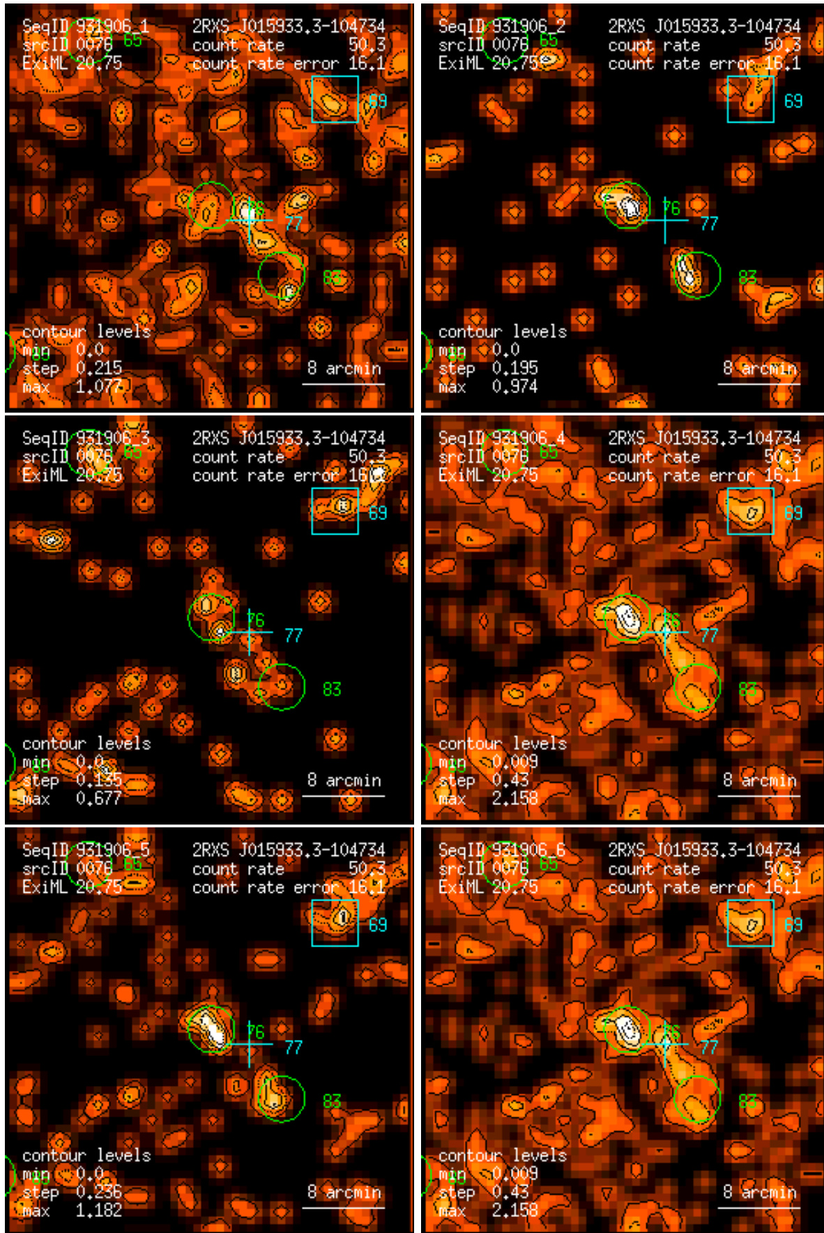
Figure 76: RASS 931906: detection 0076: band rate images, Gaussian filter: (1) PSPC channels 11 – 41, (2) 52 – 90, (3) 91 – 201, (4) 11 – 235, (5) 52 – 201, (6) 11 – 201. Broad band rates in counts/ks. Band rate contour levels in counts/ks/arcmin 2 .
