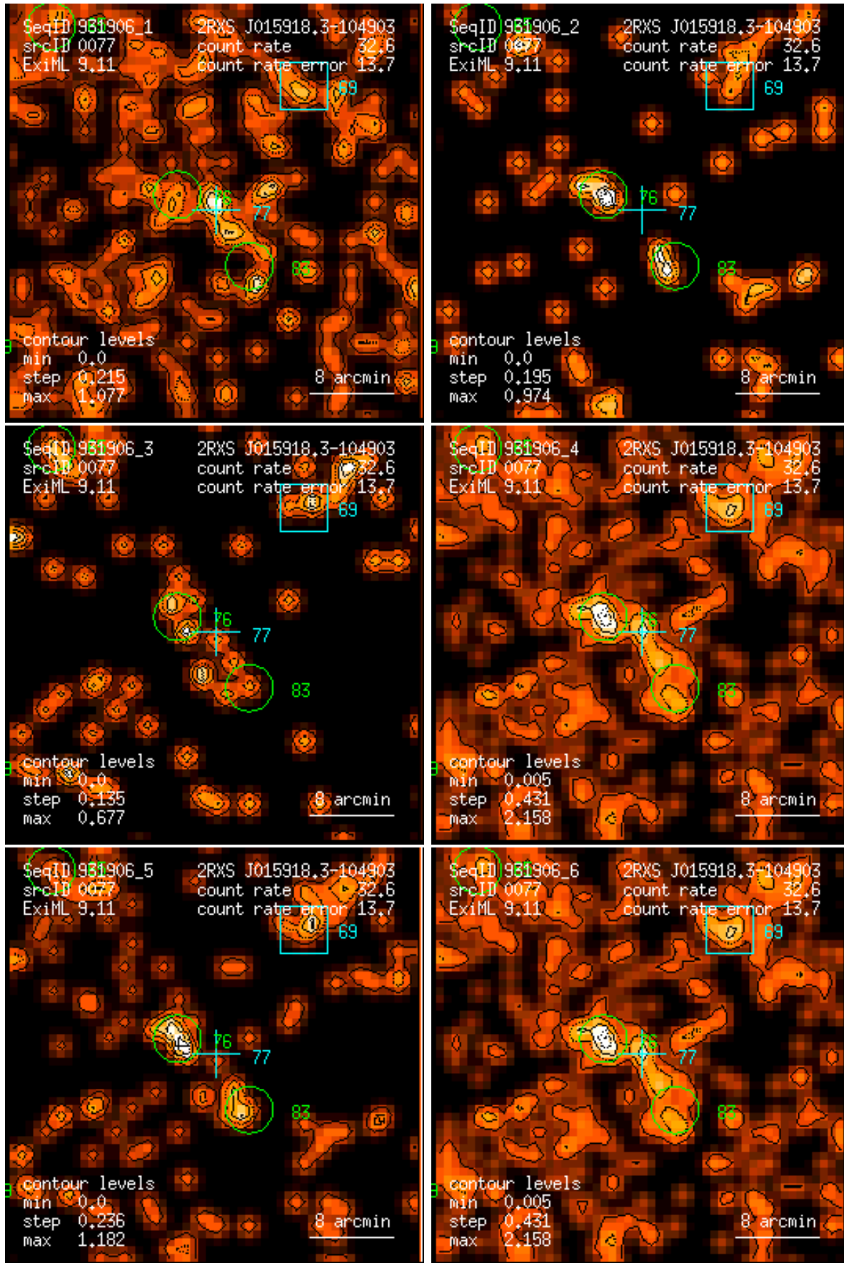
Figure 77: RASS 931906: detection 0077: band rate images, Gaussian filter: (1) PSPC channels 11 – 41, (2) 52 – 90, (3) 91 – 201, (4) 11 – 235, (5) 52 – 201, (6) 11 – 201. Broad band rates in counts/ks. Band rate contour levels in counts/ks/arcmin 2 .
