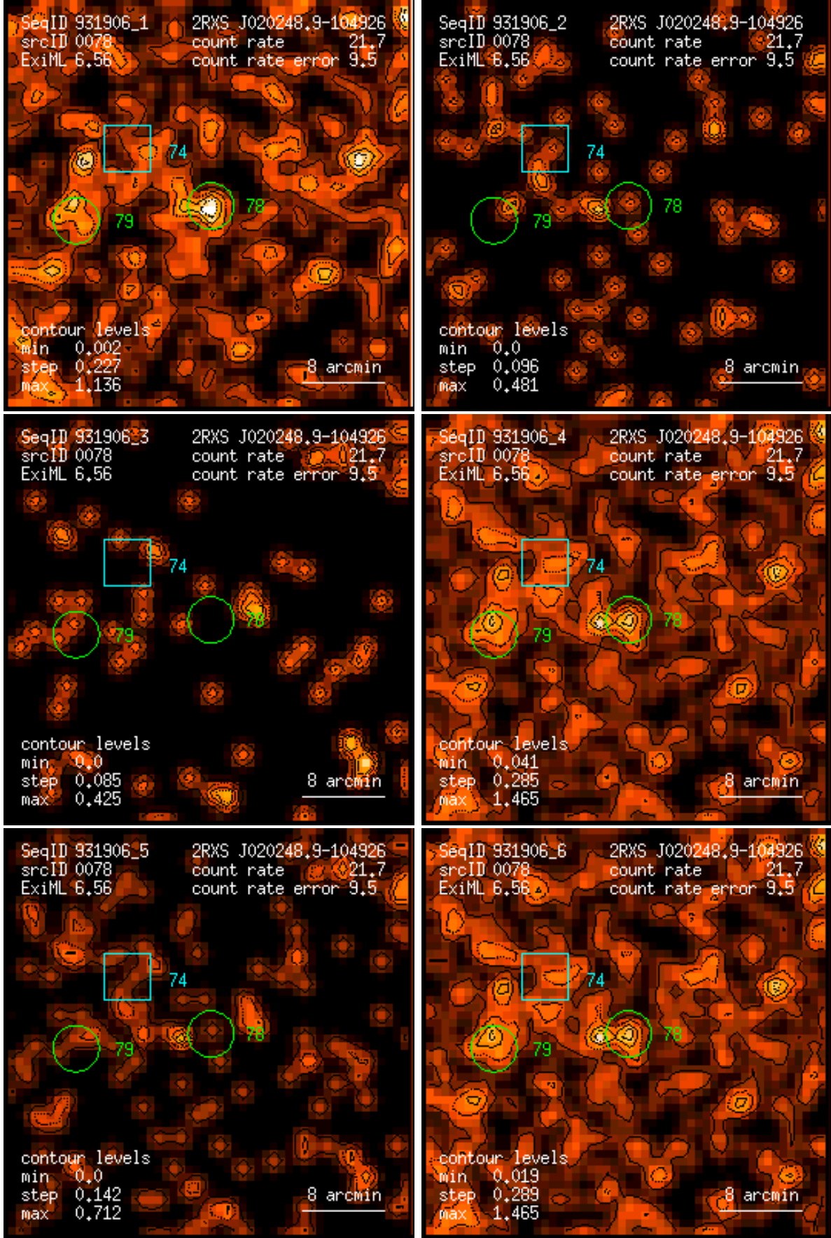
Figure 78: RASS 931906: detection 0078: band rate images, Gaussian filter: (1) PSPC channels 11 – 41, (2) 52 – 90, (3) 91 – 201, (4) 11 – 235, (5) 52 – 201, (6) 11 – 201. Broad band rates in counts/ks. Band rate contour levels in counts/ks/arcmin 2 .
