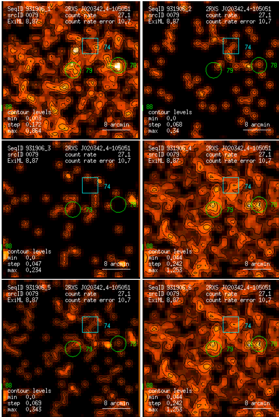
Figure 79: RASS 931906: detection 0079: band rate images, Gaussian filter: (1) PSPC channels 11 – 41, (2) 52 – 90, (3) 91 – 201, (4) 11 – 235, (5) 52 – 201, (6) 11 – 201. Broad band rates in counts/ks. Band rate contour levels in counts/ks/arcmin 2 .
