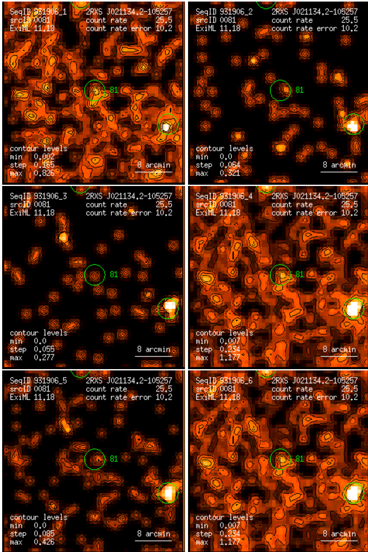
Figure 81: RASS 931906: detection 0081: band rate images, Gaussian filter: (1) PSPC channels 11 – 41, (2) 52 – 90, (3) 91 – 201, (4) 11 – 235, (5) 52 – 201, (6) 11 – 201. Broad band rates in counts/ks. Band rate contour levels in counts/ks/arcmin 2 .
