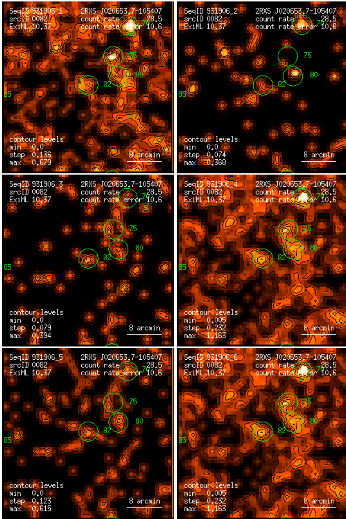
Figure 82: RASS 931906: detection 0082: band rate images, Gaussian filter: (1) PSPC channels 11 – 41, (2) 52 – 90, (3) 91 – 201, (4) 11 – 235, (5) 52 – 201, (6) 11 – 201. Broad band rates in counts/ks. Band rate contour levels in counts/ks/arcmin 2 .
