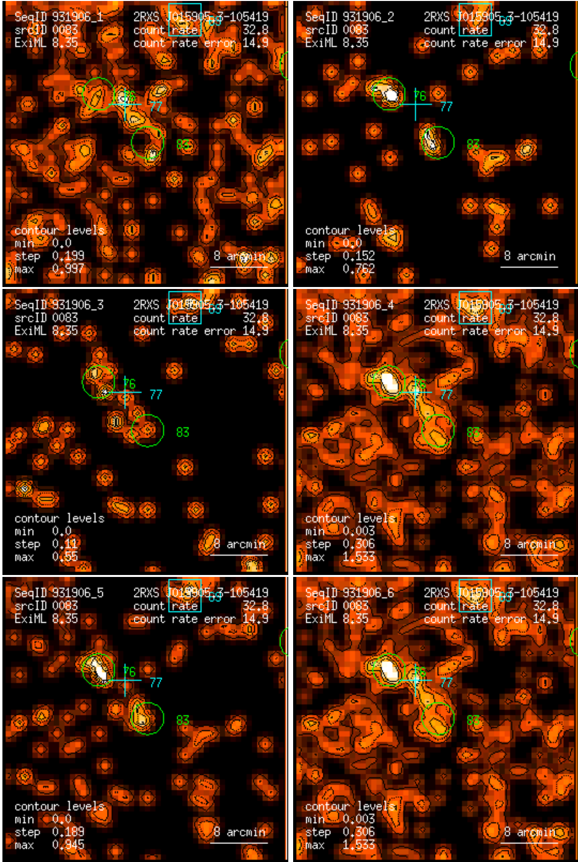
Figure 83: RASS 931906: detection 0083: band rate images, Gaussian filter: (1) PSPC channels 11 – 41, (2) 52 – 90, (3) 91 – 201, (4) 11 – 235, (5) 52 – 201, (6) 11 – 201. Broad band rates in counts/ks. Band rate contour levels in counts/ks/arcmin 2 .
