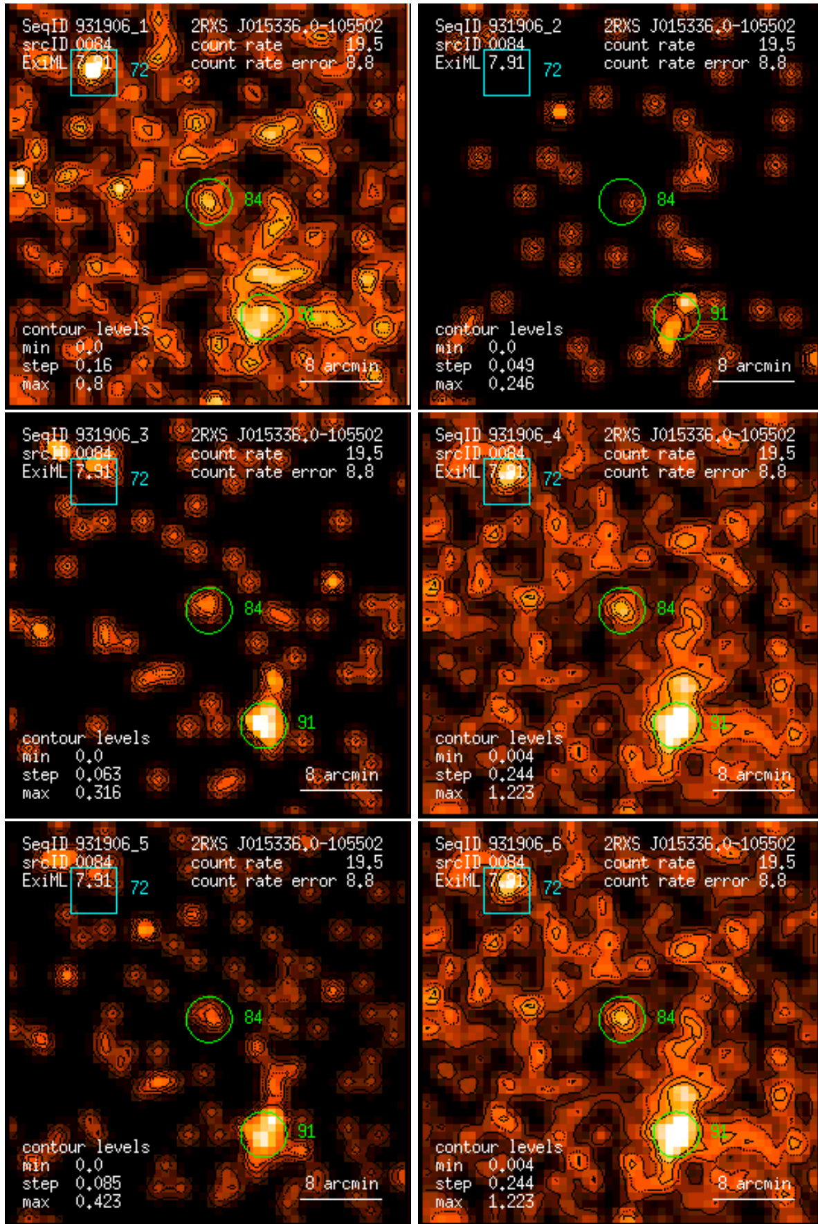
Figure 84: RASS 931906: detection 0084: band rate images, Gaussian filter: (1) PSPC channels 11 – 41, (2) 52 – 90, (3) 91 – 201, (4) 11 – 235, (5) 52 – 201, (6) 11 – 201. Broad band rates in counts/ks. Band rate contour levels in counts/ks/arcmin 2 .
