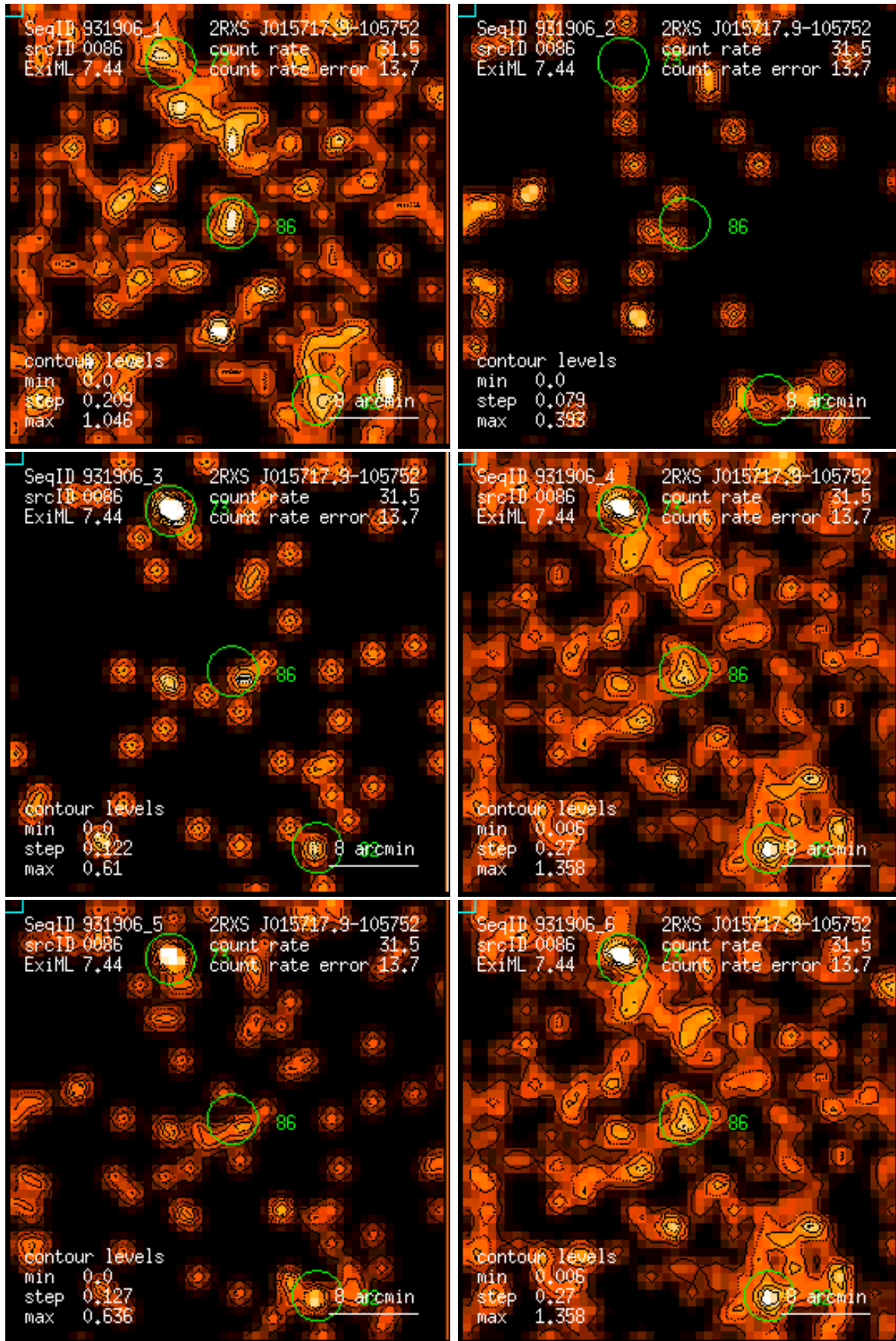
Figure 86: RASS 931906: detection 0086: band rate images, Gaussian filter: (1) PSPC channels 11 – 41, (2) 52 – 90, (3) 91 – 201, (4) 11 – 235, (5) 52 – 201, (6) 11 – 201. Broad band rates in counts/ks. Band rate contour levels in counts/ks/arcmin 2 .
