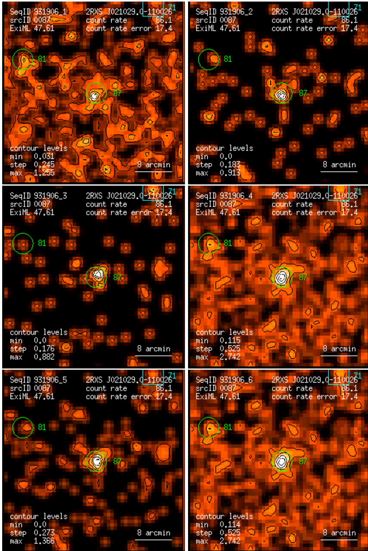
Figure 87: RASS 931906: detection 0087: band rate images, Gaussian filter: (1) PSPC channels 11 – 41, (2) 52 – 90, (3) 91 – 201, (4) 11 – 235, (5) 52 – 201, (6) 11 – 201. Broad band rates in counts/ks. Band rate contour levels in counts/ks/arcmin 2 .
