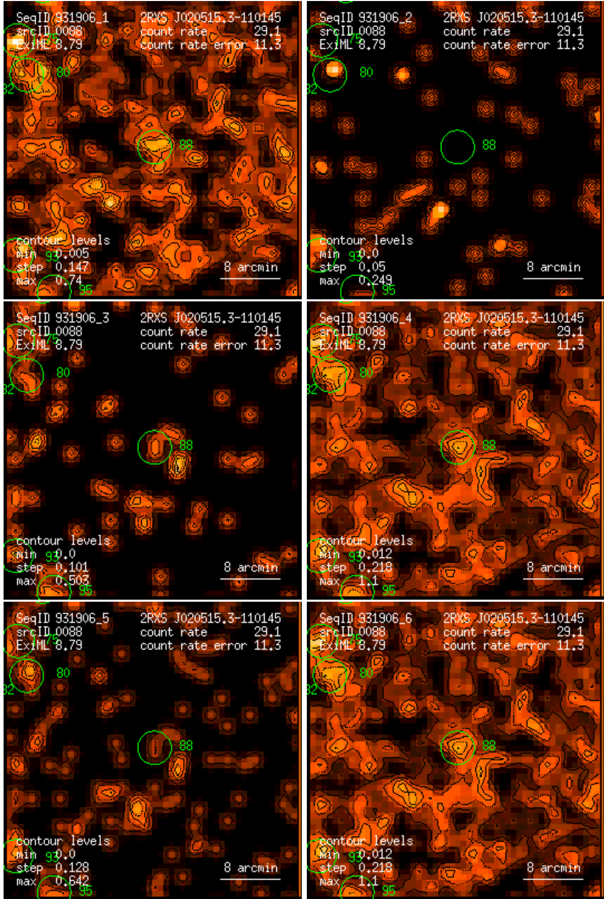
Figure 88: RASS 931906: detection 0088: band rate images, Gaussian filter: (1) PSPC channels 11 – 41, (2) 52 – 90, (3) 91 – 201, (4) 11 – 235, (5) 52 – 201, (6) 11 – 201. Broad band rates in counts/ks. Band rate contour levels in counts/ks/arcmin 2 .
