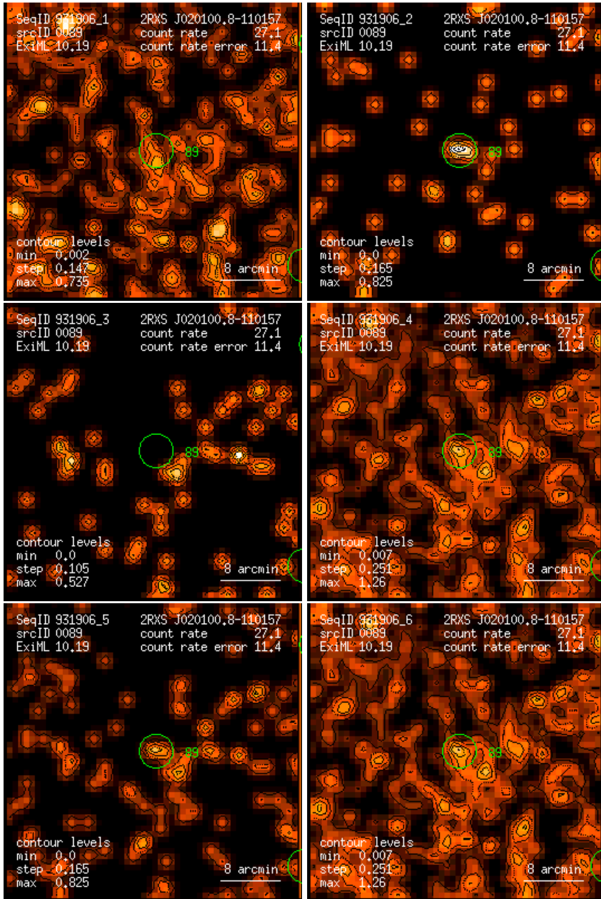
Figure 89: RASS 931906: detection 0089: band rate images, Gaussian filter: (1) PSPC channels 11 – 41, (2) 52 – 90, (3) 91 – 201, (4) 11 – 235, (5) 52 – 201, (6) 11 – 201. Broad band rates in counts/ks. Band rate contour levels in counts/ks/arcmin 2 .
