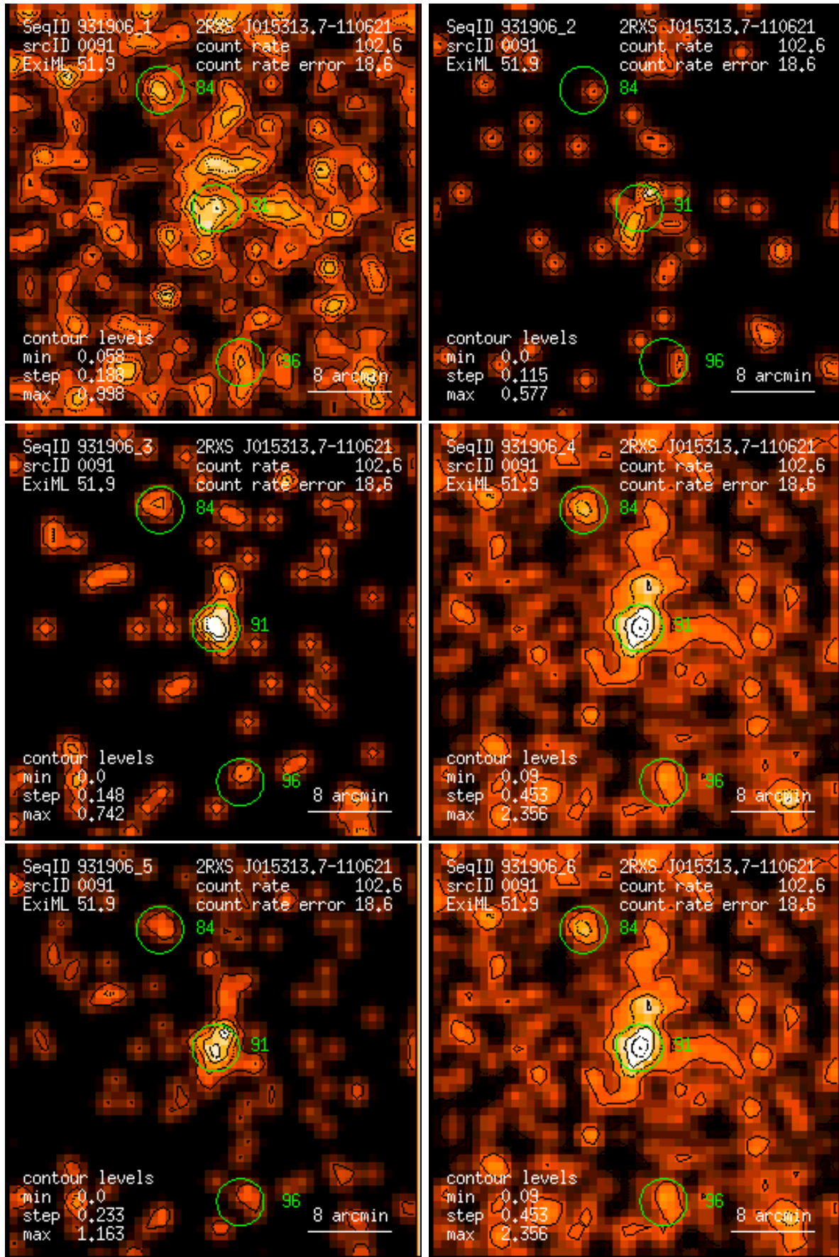
Figure 91: RASS 931906: detection 0091: band rate images, Gaussian filter: (1) PSPC channels 11 – 41, (2) 52 – 90, (3) 91 – 201, (4) 11 – 235, (5) 52 – 201, (6) 11 – 201. Broad band rates in counts/ks. Band rate contour levels in counts/ks/arcmin 2 .
