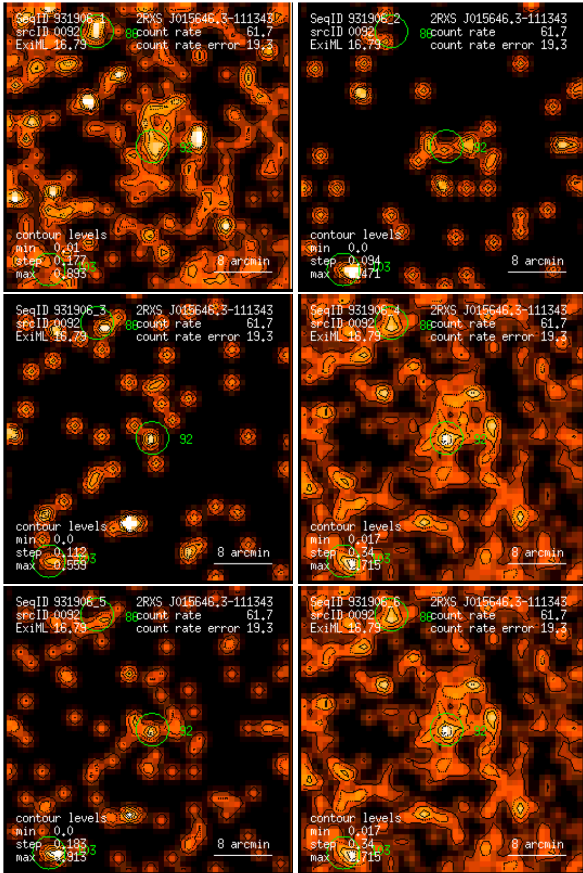
Figure 92: RASS 931906: detection 0092: band rate images, Gaussian filter: (1) PSPC channels 11 – 41, (2) 52 – 90, (3) 91 – 201, (4) 11 – 235, (5) 52 – 201, (6) 11 – 201. Broad band rates in counts/ks. Band rate contour levels in counts/ks/arcmin 2 .
