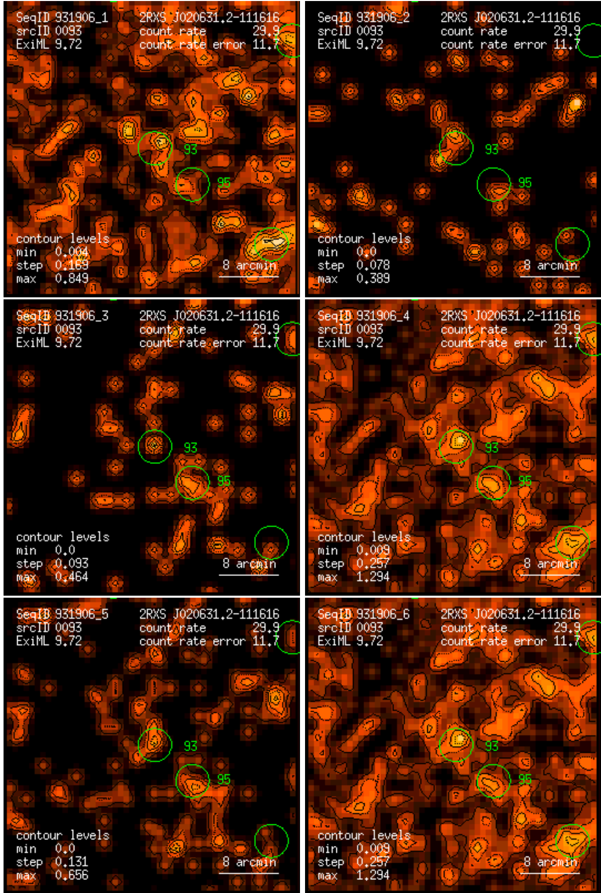
Figure 93: RASS 931906: detection 0093: band rate images, Gaussian filter: (1) PSPC channels 11 – 41, (2) 52 – 90, (3) 91 – 201, (4) 11 – 235, (5) 52 – 201, (6) 11 – 201. Broad band rates in counts/ks. Band rate contour levels in counts/ks/arcmin 2 .
