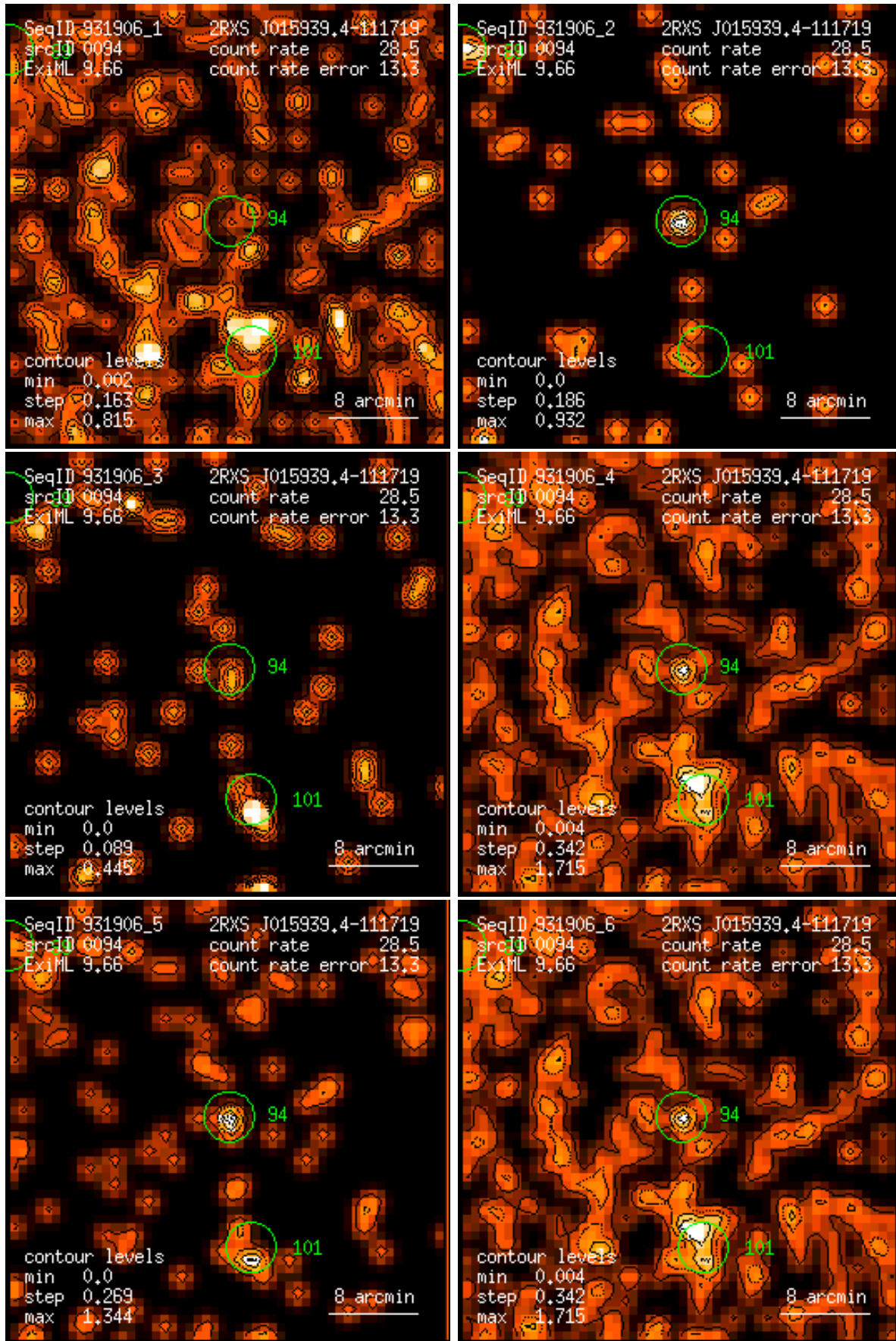
Figure 94: RASS 931906: detection 0094: band rate images, Gaussian filter: (1) PSPC channels 11 – 41, (2) 52 – 90, (3) 91 – 201, (4) 11 – 235, (5) 52 – 201, (6) 11 – 201. Broad band rates in counts/ks. Band rate contour levels in counts/ks/arcmin 2 .
