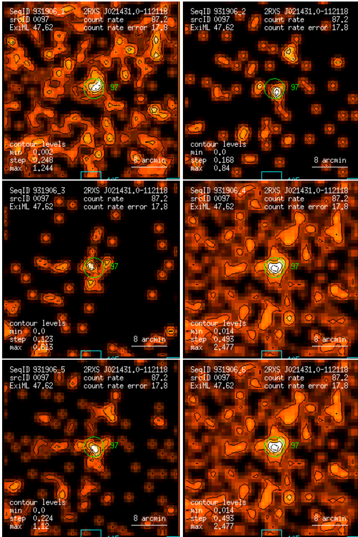
Figure 97: RASS 931906: detection 0097: band rate images, Gaussian filter: (1) PSPC channels 11 – 41, (2) 52 – 90, (3) 91 – 201, (4) 11 – 235, (5) 52 – 201, (6) 11 – 201. Broad band rates in counts/ks. Band rate contour levels in counts/ks/arcmin 2 .
