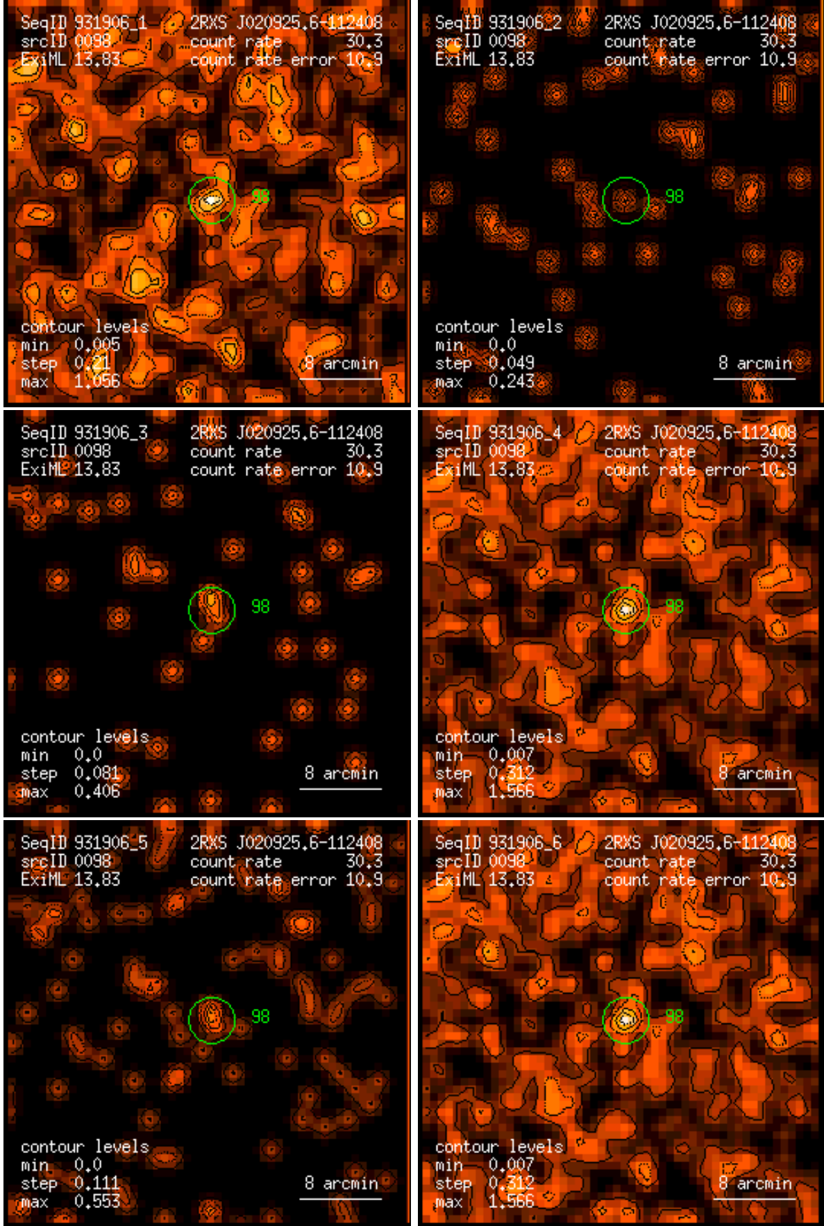
Figure 98: RASS 931906: detection 0098: band rate images, Gaussian filter: (1) PSPC channels 11 – 41, (2) 52 – 90, (3) 91 – 201, (4) 11 – 235, (5) 52 – 201, (6) 11 – 201. Broad band rates in counts/ks. Band rate contour levels in counts/ks/arcmin 2 .
