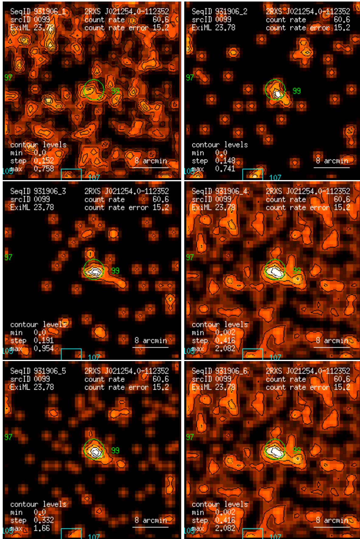
Figure 99: RASS 931906: detection 0099: band rate images, Gaussian filter: (1) PSPC channels 11 – 41, (2) 52 – 90, (3) 91 – 201, (4) 11 – 235, (5) 52 – 201, (6) 11 – 201. Broad band rates in counts/ks. Band rate contour levels in counts/ks/arcmin 2 .
