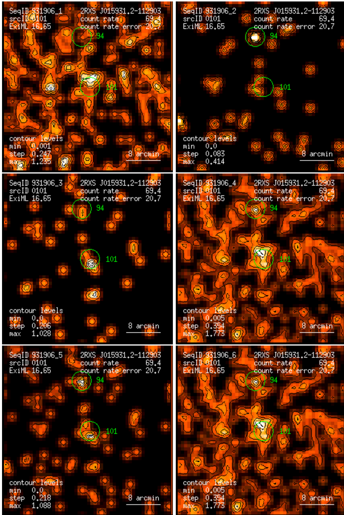
Figure 101: RASS 931906: detection 0101: band rate images, Gaussian filter: (1) PSPC channels 11 – 41, (2) 52 – 90, (3) 91 – 201, (4) 11 – 235, (5) 52 – 201, (6) 11 – 201. Broad band rates in counts/ks. Band rate contour levels in counts/ks/arcmin 2 .
