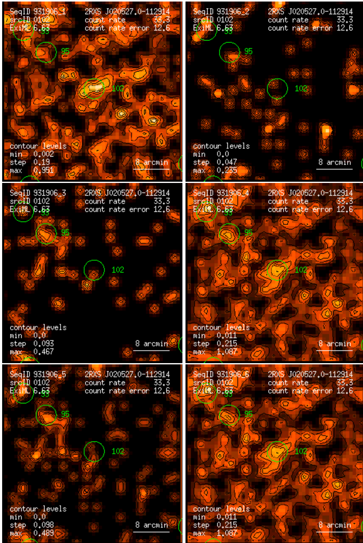
Figure 102: RASS 931906: detection 0102: band rate images, Gaussian filter: (1) PSPC channels 11 – 41, (2) 52 – 90, (3) 91 – 201, (4) 11 – 235, (5) 52 – 201, (6) 11 – 201. Broad band rates in counts/ks. Band rate contour levels in counts/ks/arcmin 2 .
